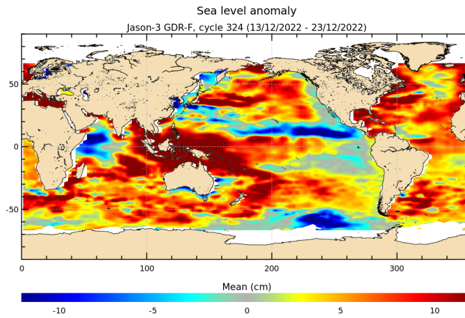
FIGURE 18 – Sea level anomaly relative to MSS for cycle 324.
