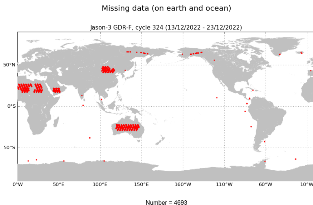
FIGURE 1 – Missing measurements for cycle 324.
