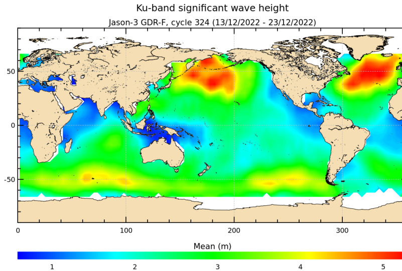
FIGURE 5 – Significant wave height for cycle 324.
