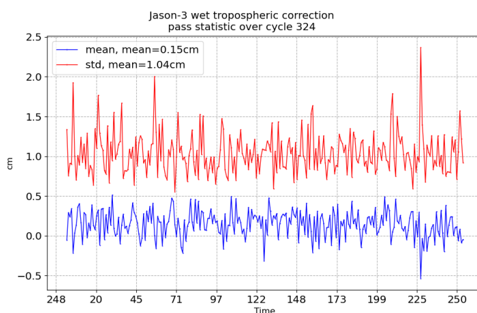
FIGURE 11 – Pass monitoring of wet troposphere differences between radiometer and ECMWF model for Jason-3 cycle 324
