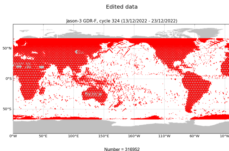
FIGURE 2 – Edited measurements for cycle 324.
