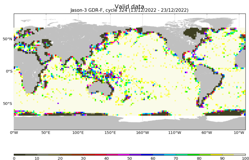
FIGURE 3 – Percentage of valid measurements for cycle 324.
