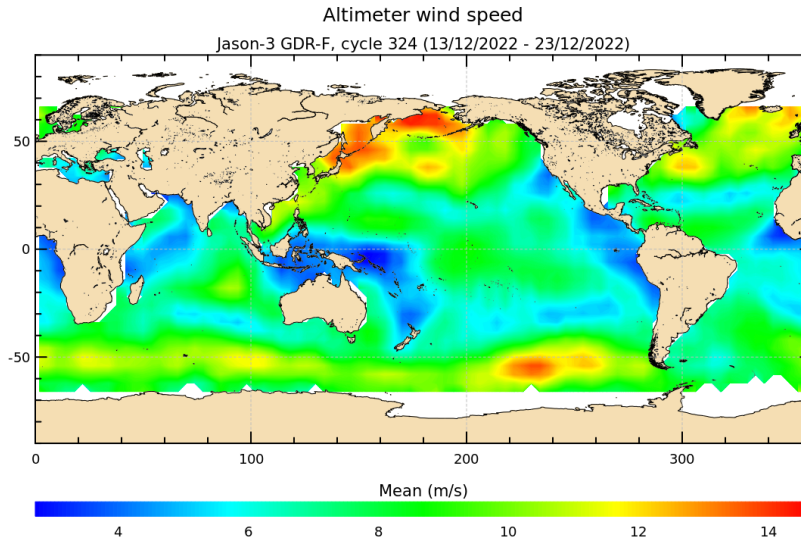
FIGURE 9 – Altimeter wind speed for cycle 324.
