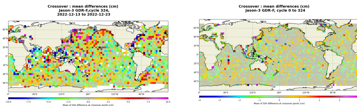
FIGURE 13 – Mean SSH at crossovers for cycle 324 (left) and over the whole Jason-3 period (right).
