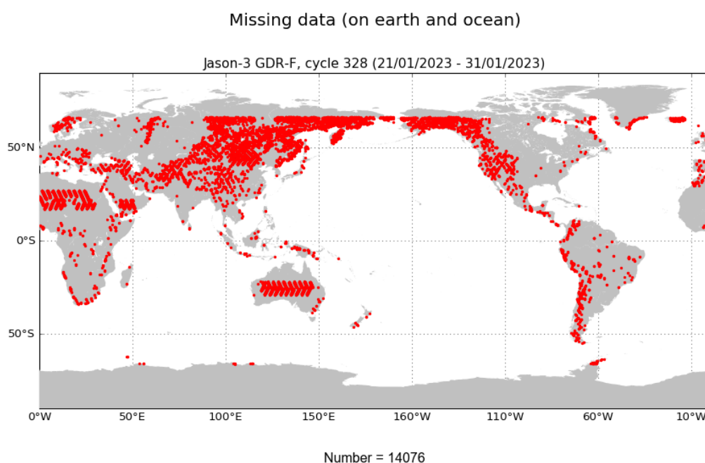
FIGURE 1 – Missing measurements for cycle 328.
