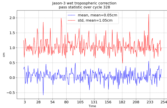
FIGURE 11 – Pass monitoring of wet troposphere differences between radiometer and ECMWF model for Jason-3 cycle 328
