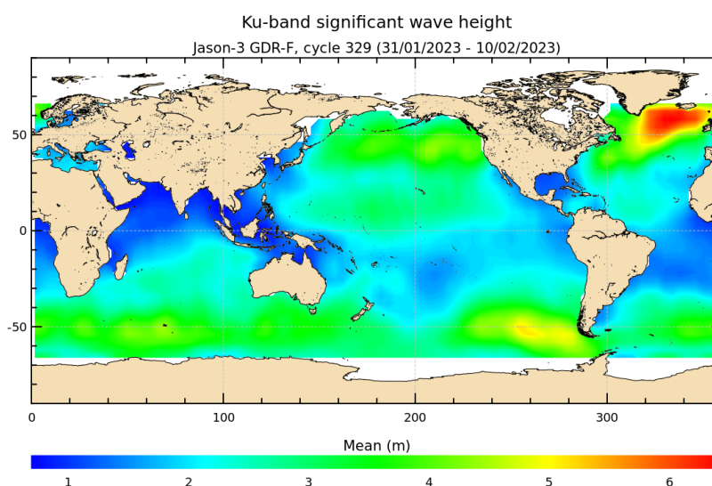
FIGURE 5 – Significant wave height for cycle 329.
