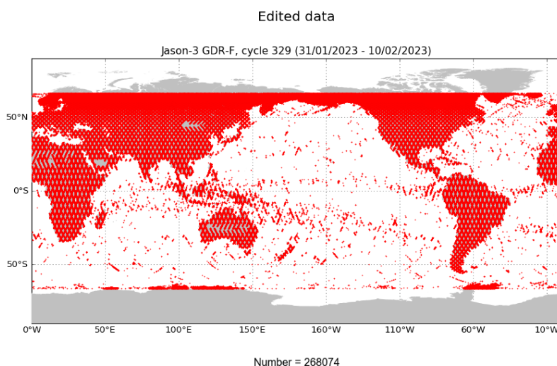
FIGURE 2 – Edited measurements for cycle 329.
