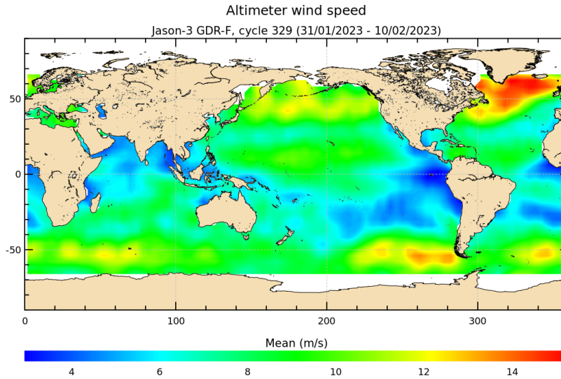
FIGURE 9 – Altimeter wind speed for cycle 329.
