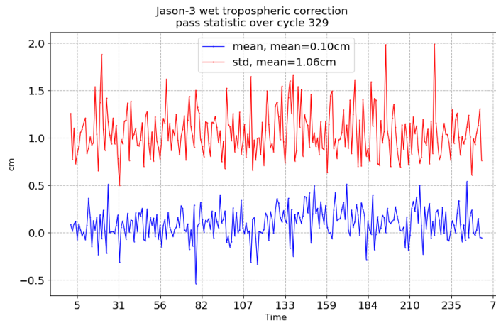
FIGURE 11 – Pass monitoring of wet troposphere differences between radiometer and ECMWF model for Jason-3 cycle 329
