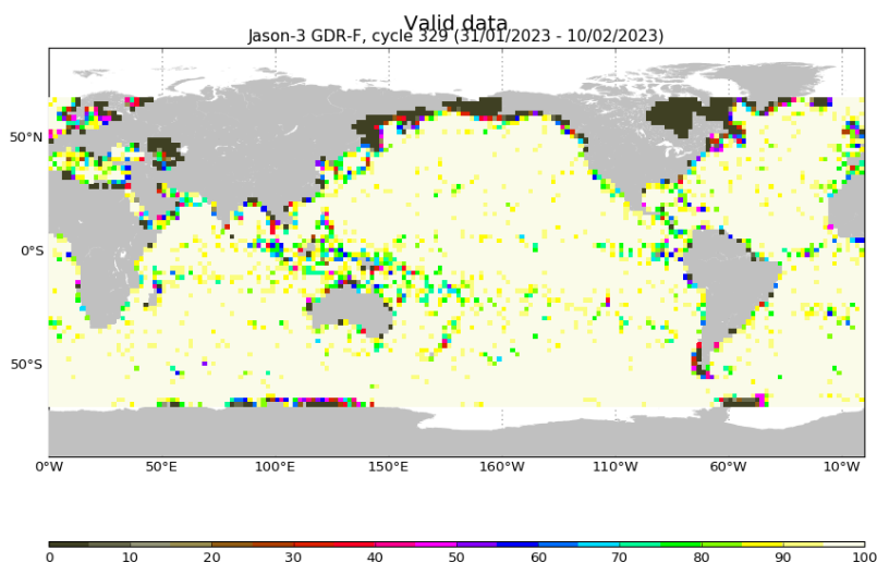
FIGURE 3 – Percentage of valid measurements for cycle 329.
