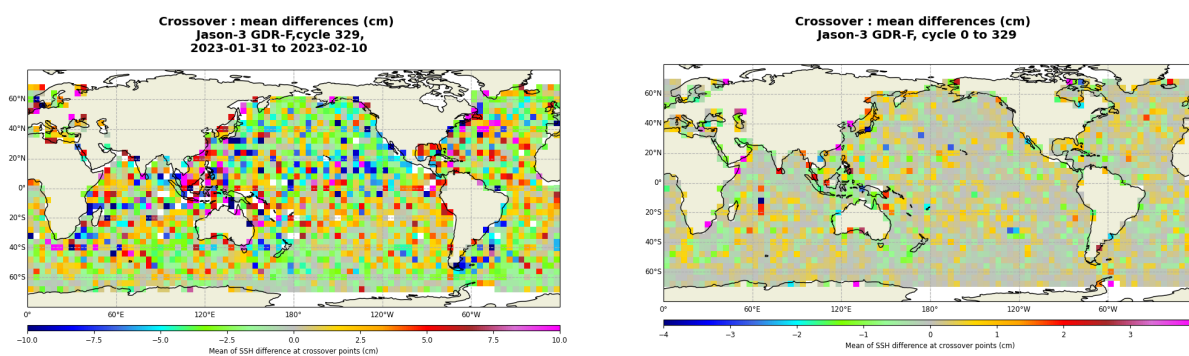
FIGURE 13 – Mean SSH at crossovers for cycle 329 (left) and over the whole Jason-3 period (right).
