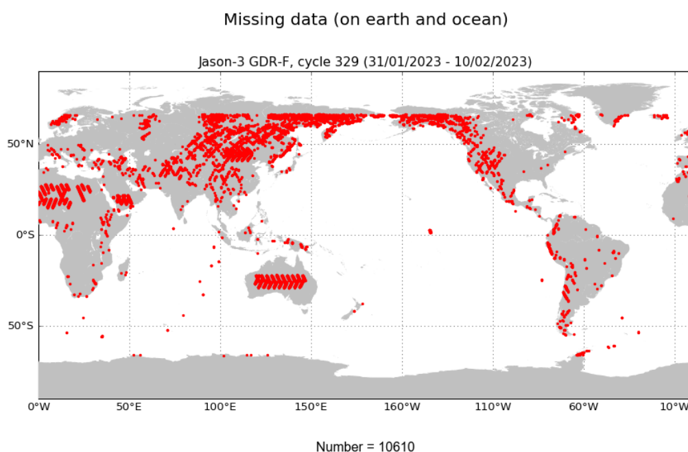
FIGURE 1 – Missing measurements for cycle 329.
