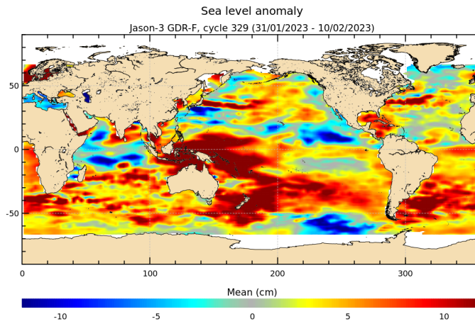
FIGURE 18 – Sea level anomaly relative to MSS for cycle 329.
