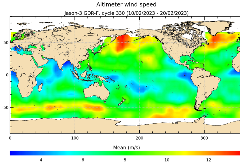
FIGURE 9 – Altimeter wind speed for cycle 330.
