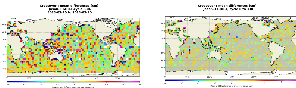
FIGURE 13 – Mean SSH at crossovers for cycle 330 (left) and over the whole Jason-3 period (right).
