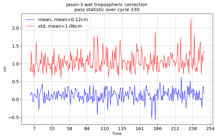
FIGURE 11 – Pass monitoring of wet troposphere differences between radiometer and ECMWF model for Jason-3 cycle 330
