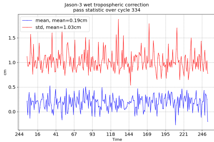
FIGURE 11 – Pass monitoring of wet troposphere differences between radiometer and ECMWF model for Jason-3 cycle 334
