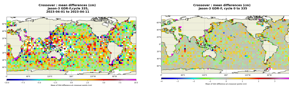
FIGURE 13 – Mean SSH at crossovers for cycle 335 (left) and over the whole Jason-3 period (right).
