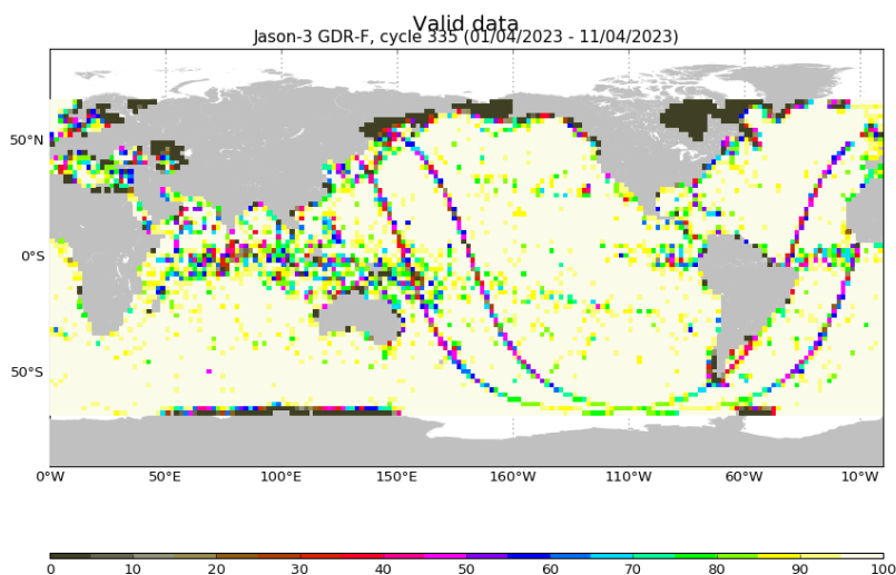
FIGURE 3 – Percentage of valid measurements for cycle 335.
