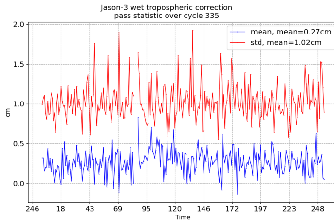
FIGURE 11 – Pass monitoring of wet troposphere differences between radiometer and ECMWF model for Jason-3 cycle 335
