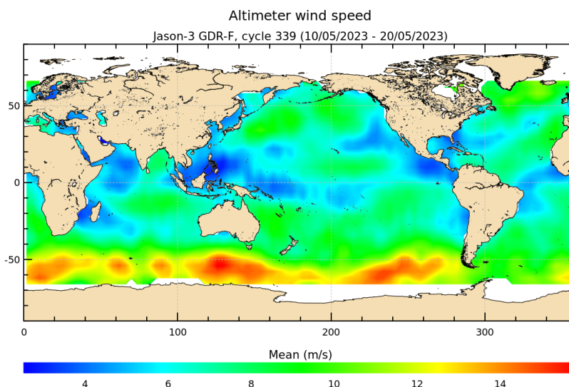
FIGURE 9 – Altimeter wind speed for cycle 339.
