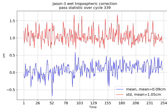
FIGURE 11 – Pass monitoring of wet troposphere differences between radiometer and ECMWF model for Jason-3 cycle 339
