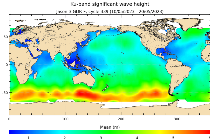
FIGURE 5 – Significant wave height for cycle 339.
