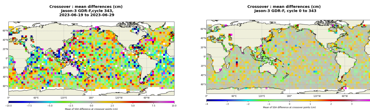
FIGURE 13 – Mean SSH at crossovers for cycle 343 (left) and over the whole Jason-3 period (right).
