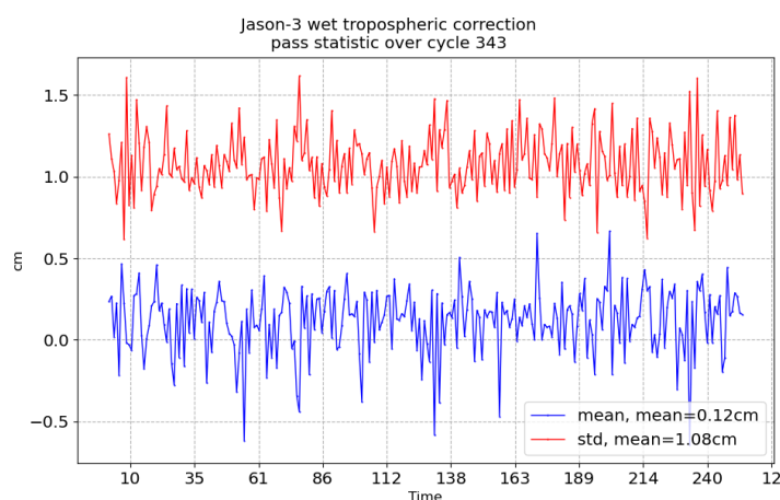
FIGURE 11 – Pass monitoring of wet troposphere differences between radiometer and ECMWF model for Jason-3 cycle 343
