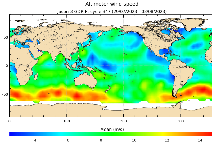
FIGURE 9 – Altimeter wind speed for cycle 347.
