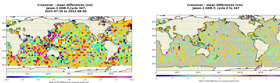
FIGURE 13 – Mean SSH at crossovers for cycle 347 (left) and over the whole Jason-3 period (right).
