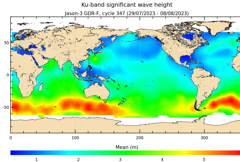
FIGURE 5 – Significant wave height for cycle 347.
