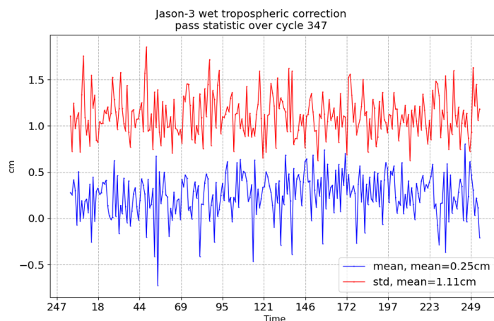
FIGURE 11 – Pass monitoring of wet troposphere differences between radiometer and ECMWF model for Jason-3 cycle 347
