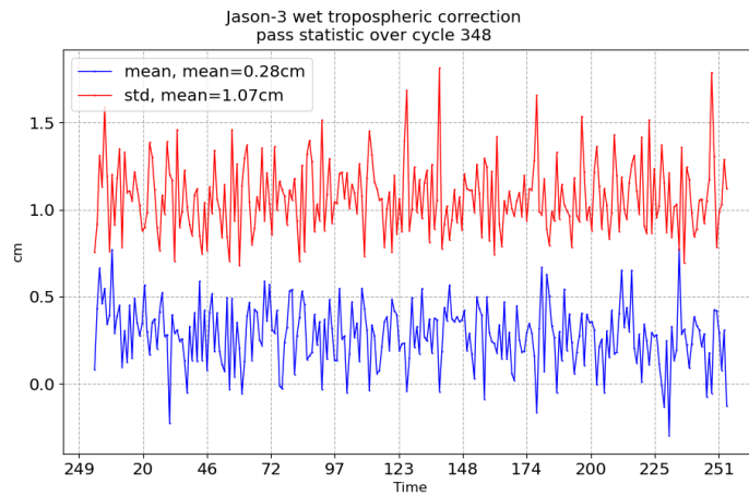
FIGURE 11 – Pass monitoring of wet troposphere differences between radiometer and ECMWF model for Jason-3 cycle 348
