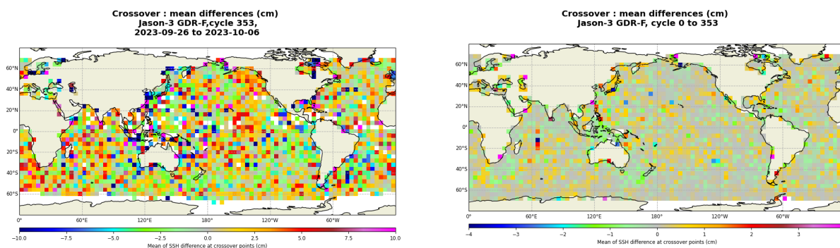
FIGURE 13 – Mean SSH at crossovers for cycle 353 (left) and over the whole Jason-3 period (right).
