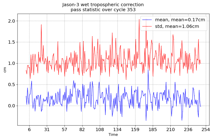
FIGURE 11 – Pass monitoring of wet troposphere differences between radiometer and ECMWF model for Jason-3 cycle 353
