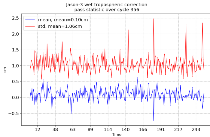
FIGURE 11 – Pass monitoring of wet troposphere differences between radiometer and ECMWF model for Jason-3 cycle 356
