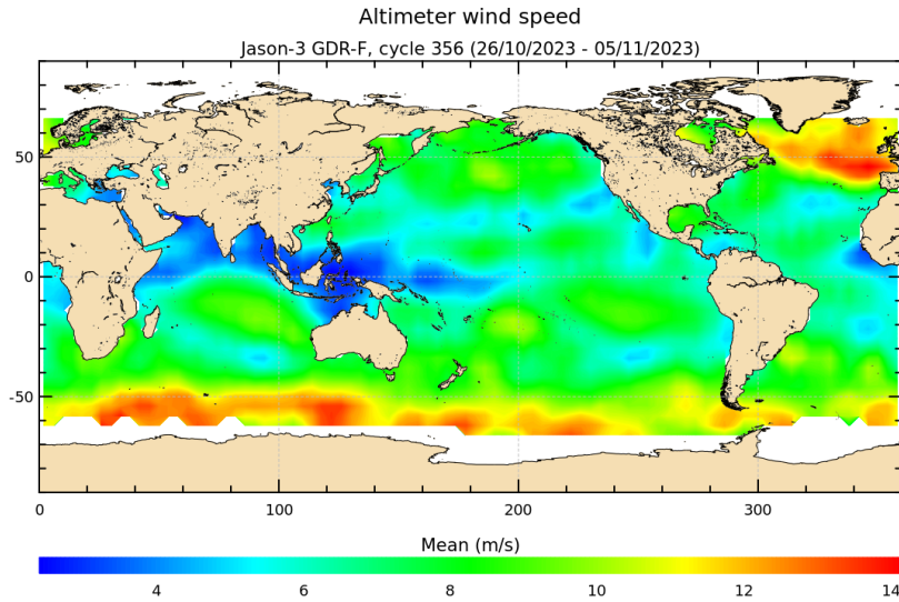
FIGURE 9 – Altimeter wind speed for cycle 356.
