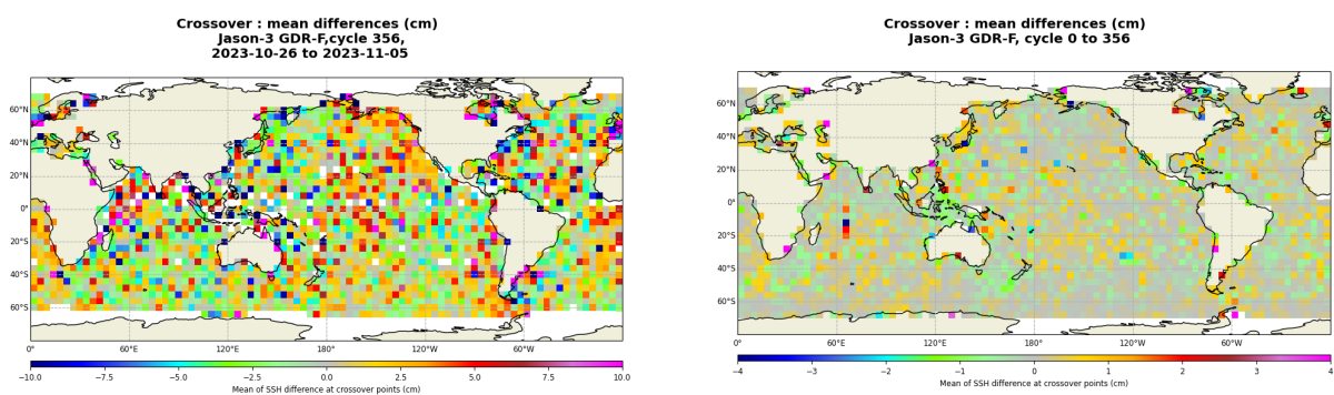
FIGURE 13 – Mean SSH at crossovers for cycle 356 (left) and over the whole Jason-3 period (right).
