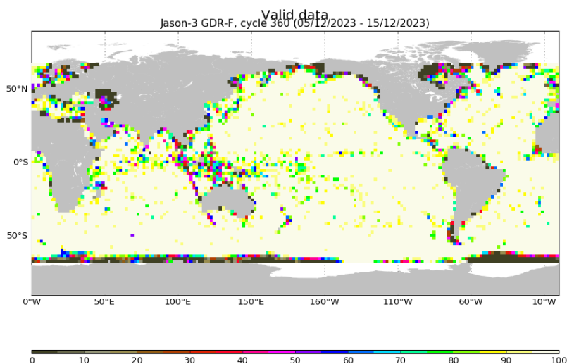
FIGURE 3 – Percentage of valid measurements for cycle 360.
