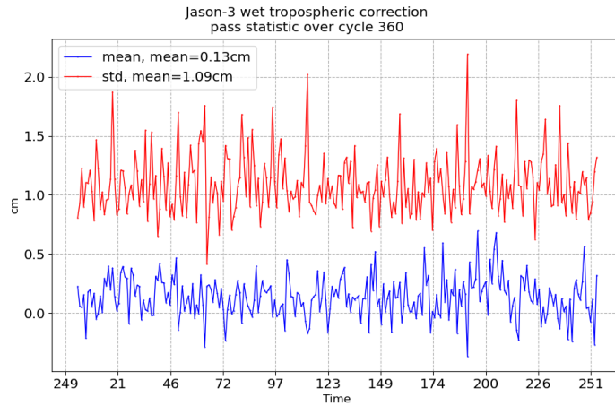
FIGURE 11 – Pass monitoring of wet troposphere differences between radiometer and ECMWF model for Jason-3 cycle 360
