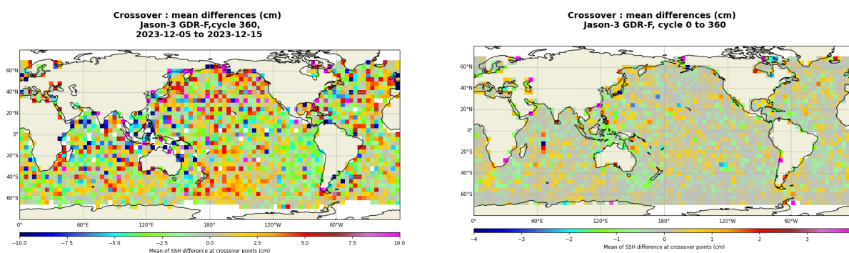
FIGURE 13 – Mean SSH at crossovers for cycle 360 (left) and over the whole Jason-3 period (right).
