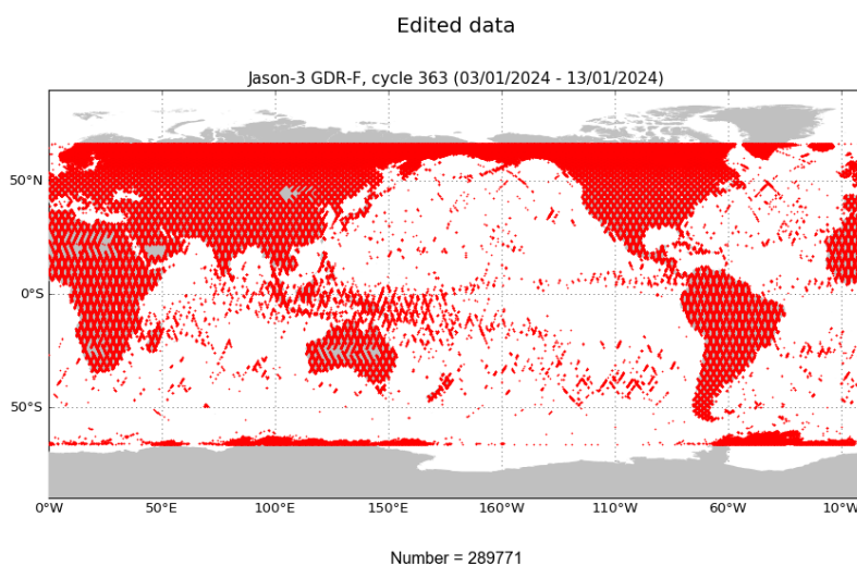
FIGURE 2 – Edited measurements for cycle 363.
