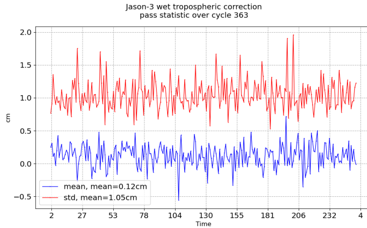
FIGURE 11 – Pass monitoring of wet troposphere differences between radiometer and ECMWF model for Jason-3 cycle 363
