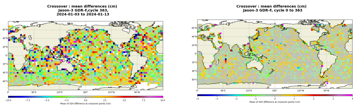
FIGURE 13 – Mean SSH at crossovers for cycle 363 (left) and over the whole Jason-3 period (right).
