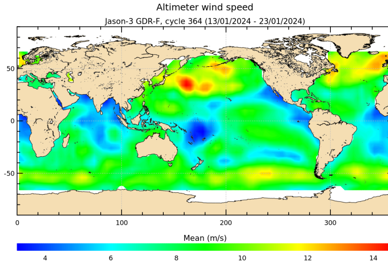
FIGURE 9 – Altimeter wind speed for cycle 364.
