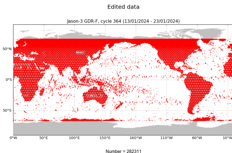
FIGURE 2 – Edited measurements for cycle 364.
