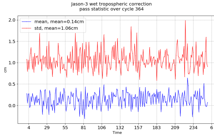
FIGURE 11 – Pass monitoring of wet troposphere differences between radiometer and ECMWF model for Jason-3 cycle 364
