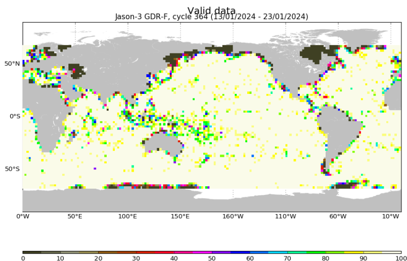
FIGURE 3 – Percentage of valid measurements for cycle 364.
