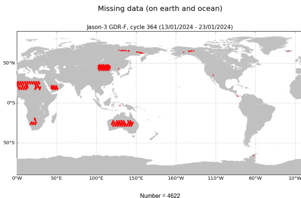
FIGURE 1 – Missing measurements for cycle 364.
