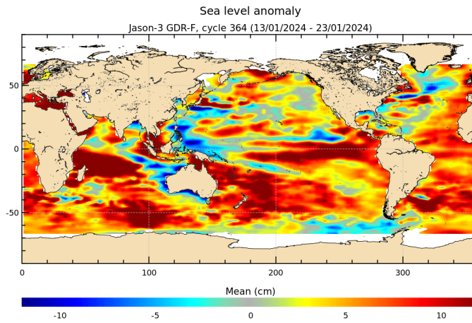
FIGURE 18 – Sea level anomaly relative to MSS for cycle 364.
