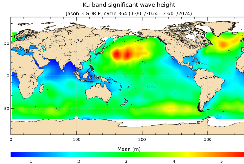
FIGURE 5 – Significant wave height for cycle 364.
