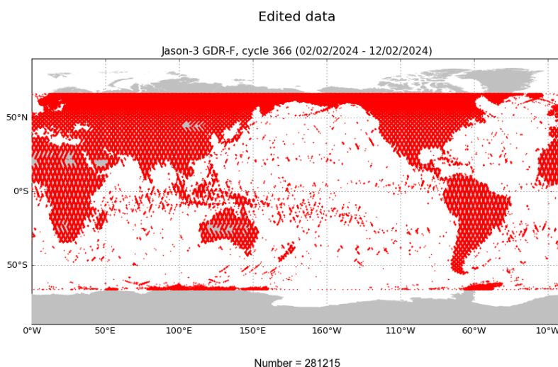
FIGURE 2 – Edited measurements for cycle 366.
