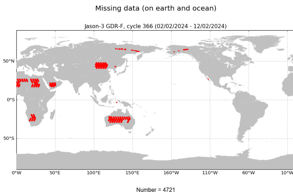
FIGURE 1 – Missing measurements for cycle 366.
