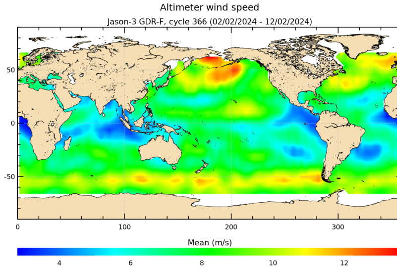
FIGURE 9 – Altimeter wind speed for cycle 366.
