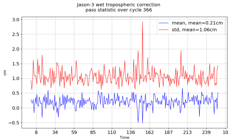
FIGURE 11 – Pass monitoring of wet troposphere differences between radiometer and ECMWF model for Jason-3 cycle 366
