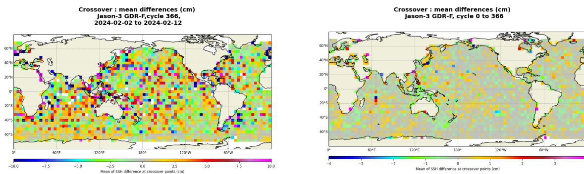
FIGURE 13 – Mean SSH at crossovers for cycle 366 (left) and over the whole Jason-3 period (right).
