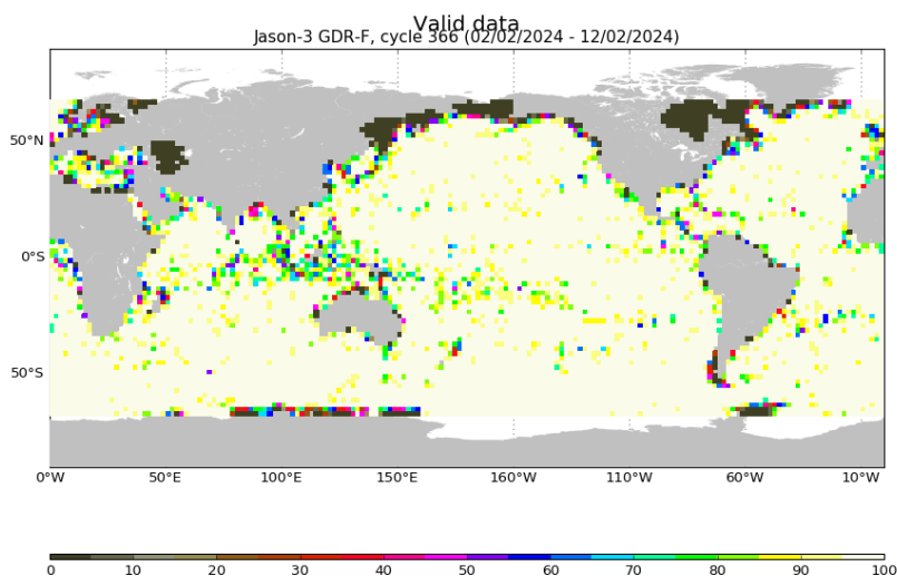
FIGURE 3 – Percentage of valid measurements for cycle 366.
