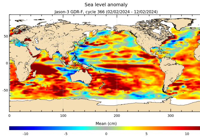
FIGURE 18 – Sea level anomaly relative to MSS for cycle 366.
