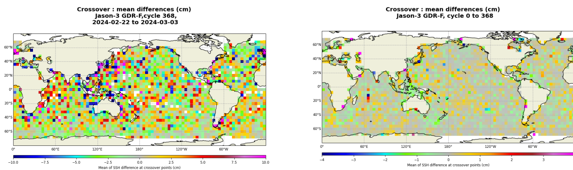
FIGURE 13 – Mean SSH at crossovers for cycle 368 (left) and over the whole Jason-3 period (right).
