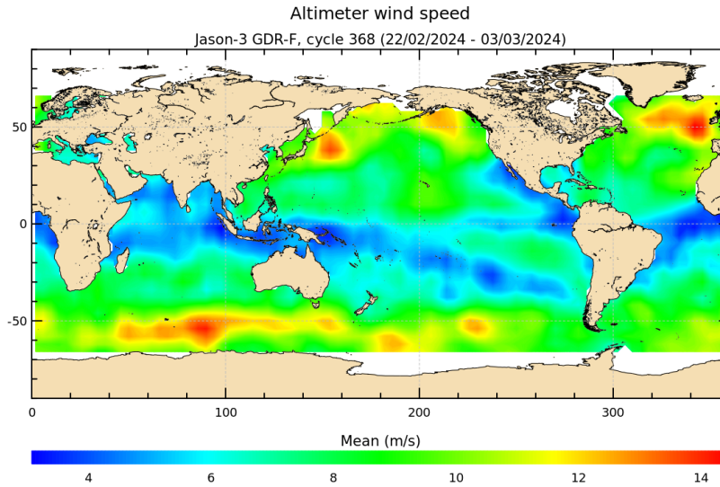
FIGURE 9 – Altimeter wind speed for cycle 368.
