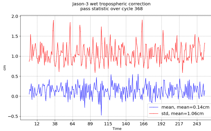
FIGURE 11 – Pass monitoring of wet troposphere differences between radiometer and ECMWF model for Jason-3 cycle 368
