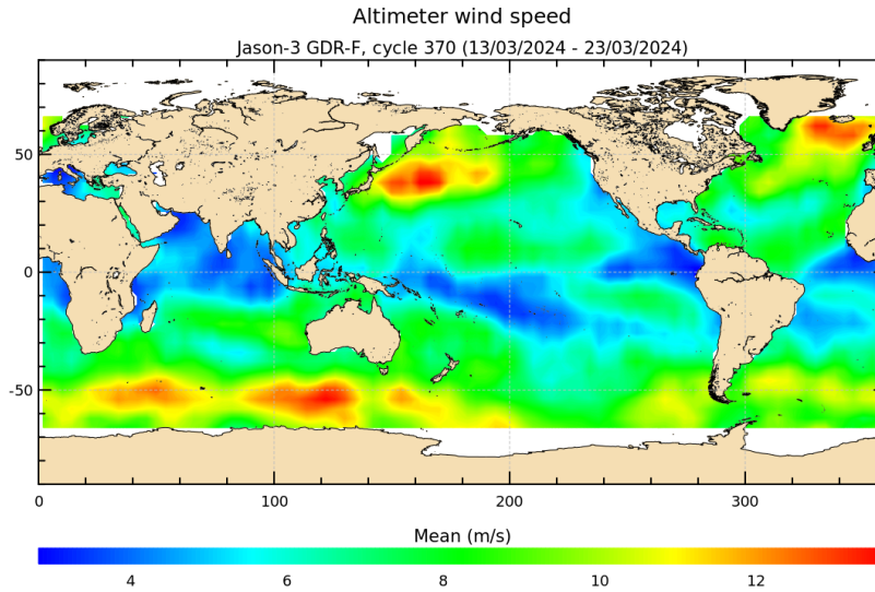
FIGURE 9 – Altimeter wind speed for cycle 370.
