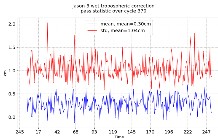
FIGURE 11 – Pass monitoring of wet troposphere differences between radiometer and ECMWF model for Jason-3 cycle 370
