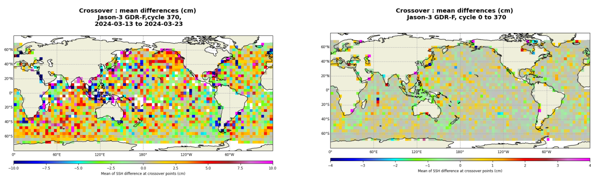
FIGURE 13 – Mean SSH at crossovers for cycle 370 (left) and over the whole Jason-3 period (right).
