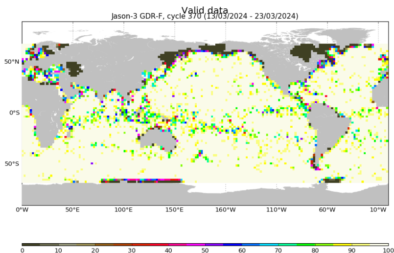
FIGURE 3 – Percentage of valid measurements for cycle 370.
