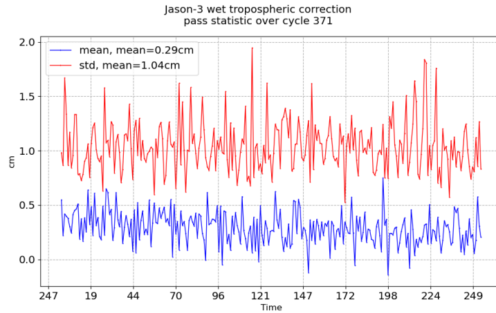
FIGURE 11 – Pass monitoring of wet troposphere differences between radiometer and ECMWF model for Jason-3 cycle 371
