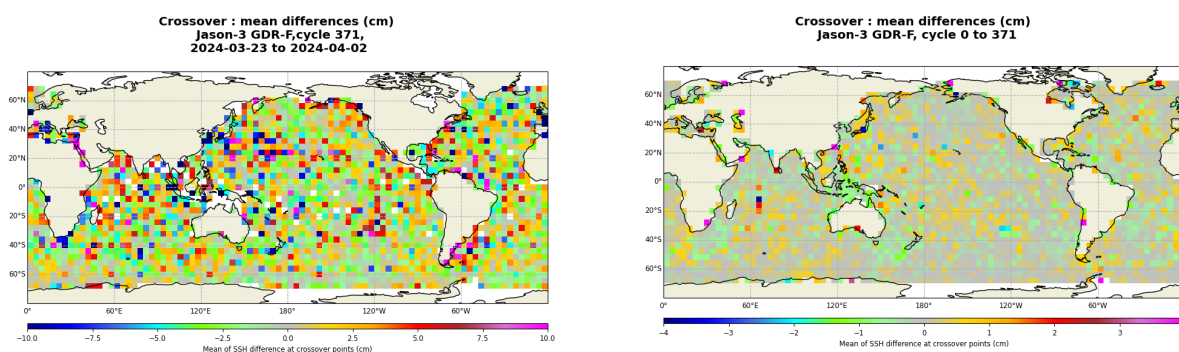
FIGURE 13 – Mean SSH at crossovers for cycle 371 (left) and over the whole Jason-3 period (right).
