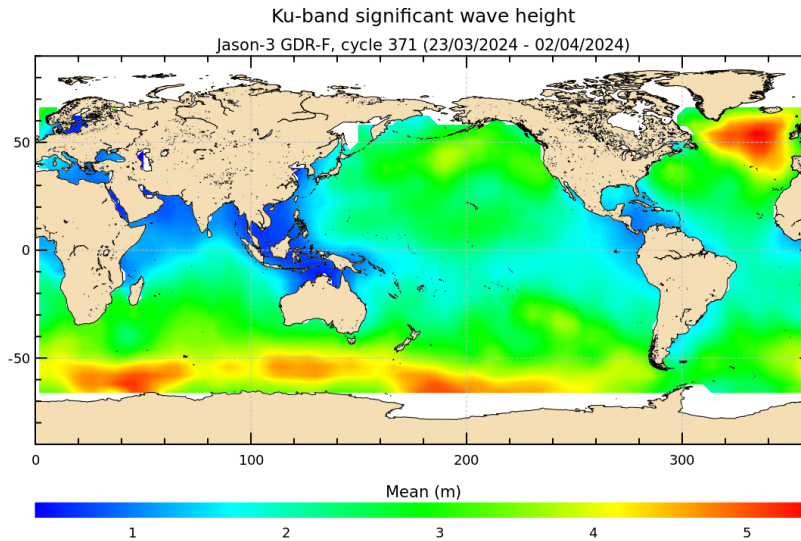
FIGURE 5 – Significant wave height for cycle 371.
