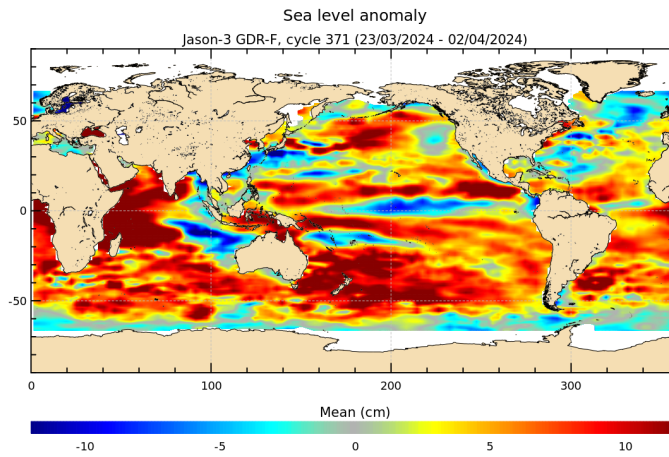
FIGURE 18 – Sea level anomaly relative to MSS for cycle 371.
