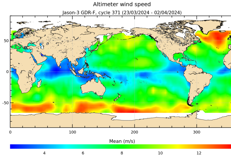
FIGURE 9 – Altimeter wind speed for cycle 371.
