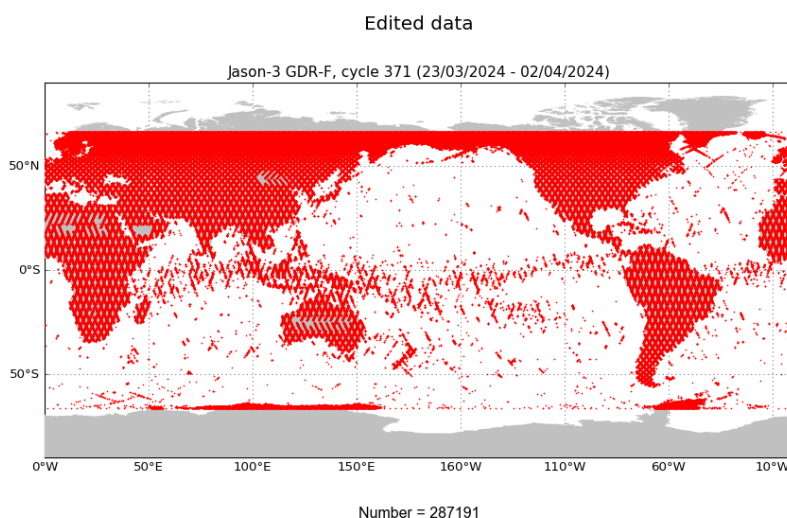
FIGURE 2 – Edited measurements for cycle 371.
