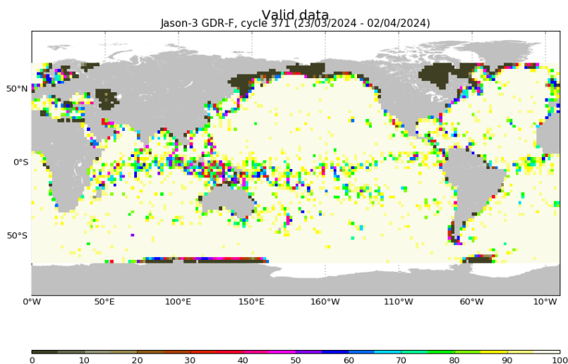
FIGURE 3 – Percentage of valid measurements for cycle 371.
