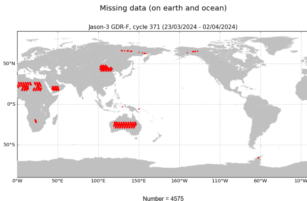
FIGURE 1 – Missing measurements for cycle 371.
