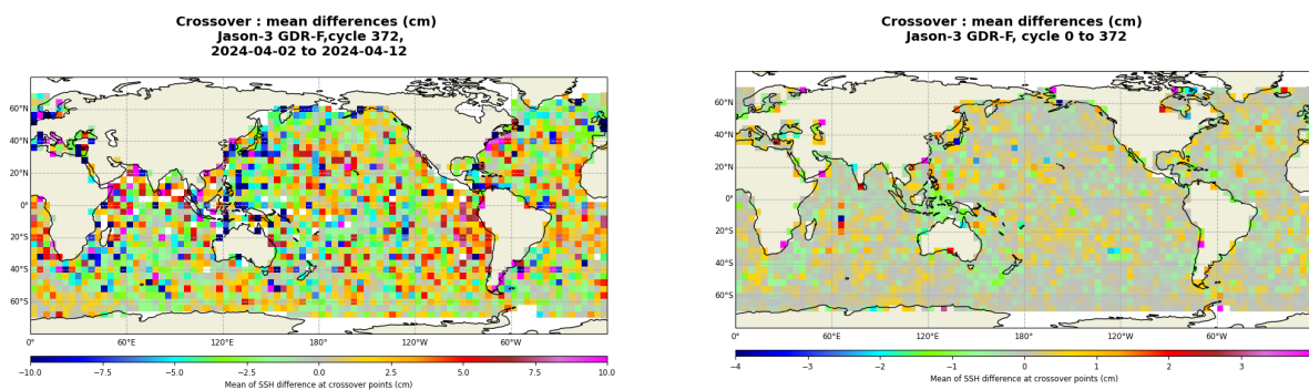
FIGURE 13 – Mean SSH at crossovers for cycle 372 (left) and over the whole Jason-3 period (right).
