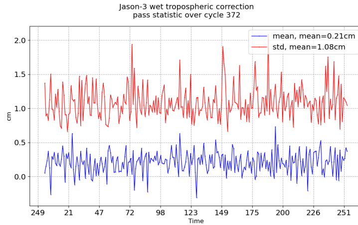
FIGURE 11 – Pass monitoring of wet troposphere differences between radiometer and ECMWF model for Jason-3 cycle 372
