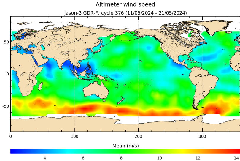
FIGURE 9 – Altimeter wind speed for cycle 376.
