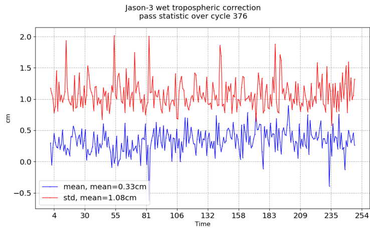
FIGURE 11 – Pass monitoring of wet troposphere differences between radiometer and ECMWF model for Jason-3 cycle 376
