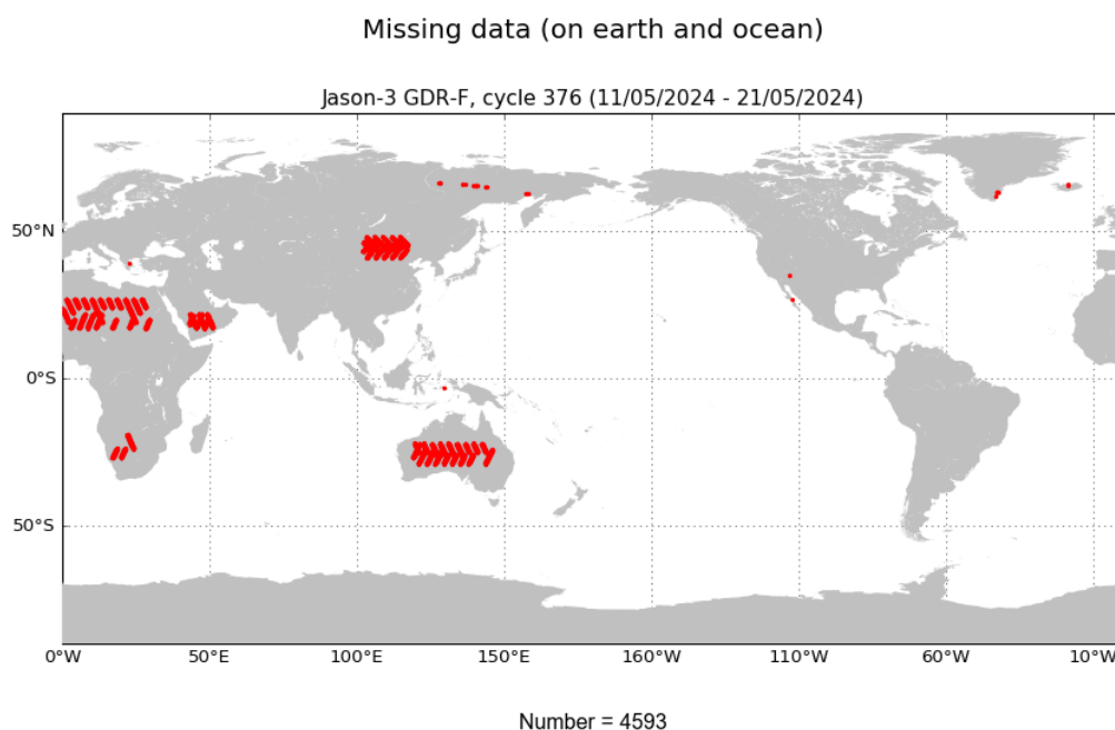
FIGURE 1 – Missing measurements for cycle 376.
