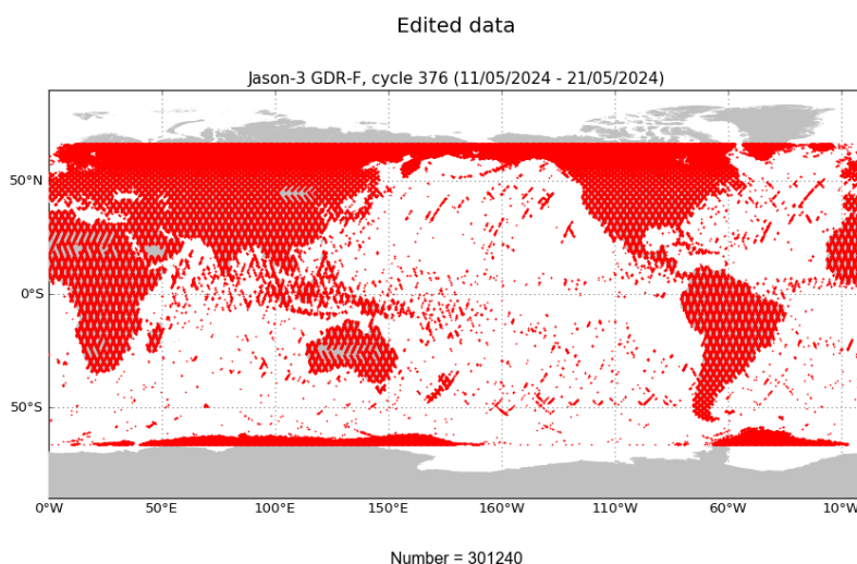
FIGURE 2 – Edited measurements for cycle 376.
