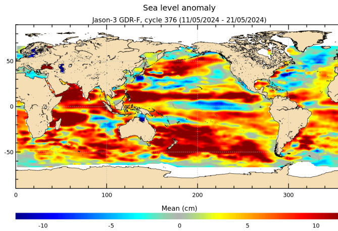
FIGURE 18 – Sea level anomaly relative to MSS for cycle 376.
