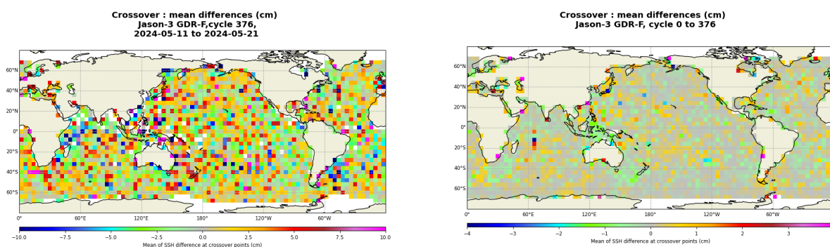
FIGURE 13 – Mean SSH at crossovers for cycle 376 (left) and over the whole Jason-3 period (right).
