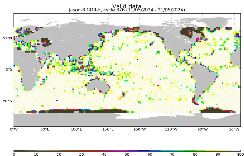
FIGURE 3 – Percentage of valid measurements for cycle 376.
