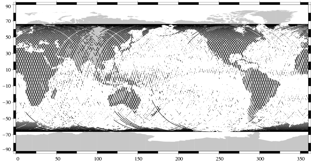
Edited measurements TOPEX Cycle 374 (08/11/2002 / 18/11/2002)
