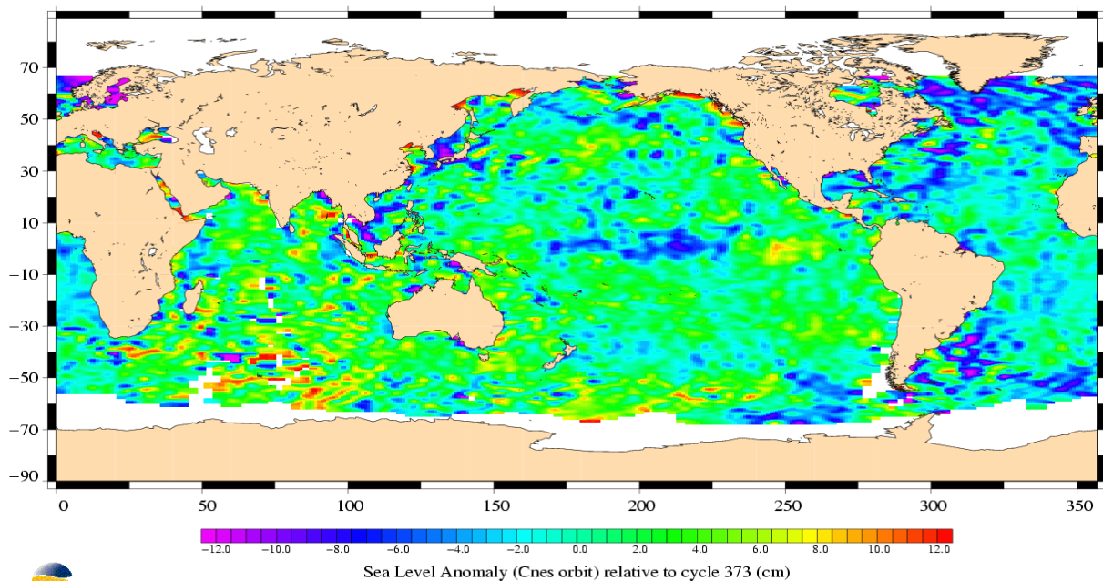
TOPEX/Poseidon, cycle 374 Period : 08/11/2002 – 18/11/2002
