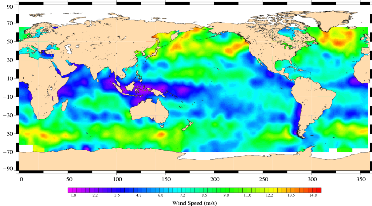
TOPEX/Poseidon, cycle 374 Period : 08/11/2002 – 18/11/2002
