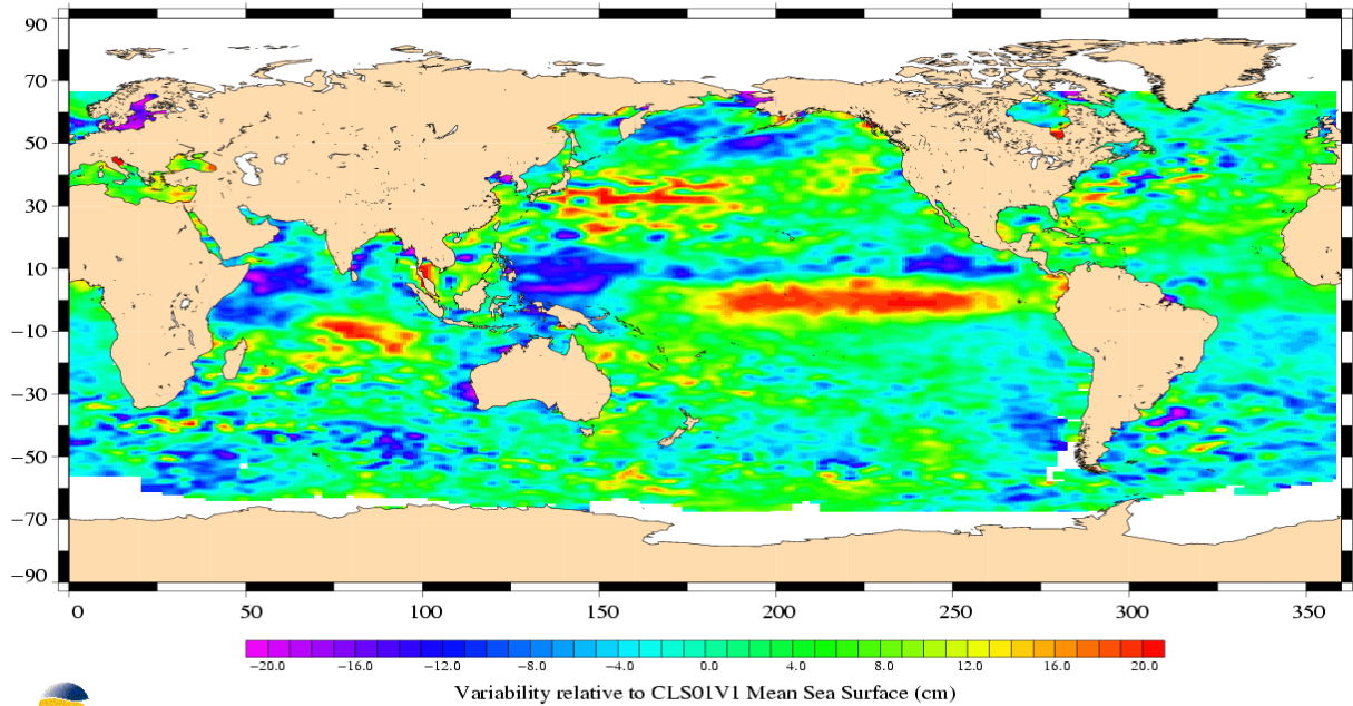
(SSH – MSS) differences greater than 0.3 m TOPEX/Poseidon Cycle 374 (08/11/2002 / 18/11/2002)
