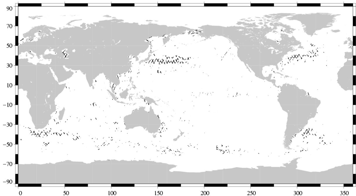
(SSH – MSS) differences greater than 0.3 m TOPEX/Poseidon Cycle 374 (08/11/2002 / 18/11/2002)
