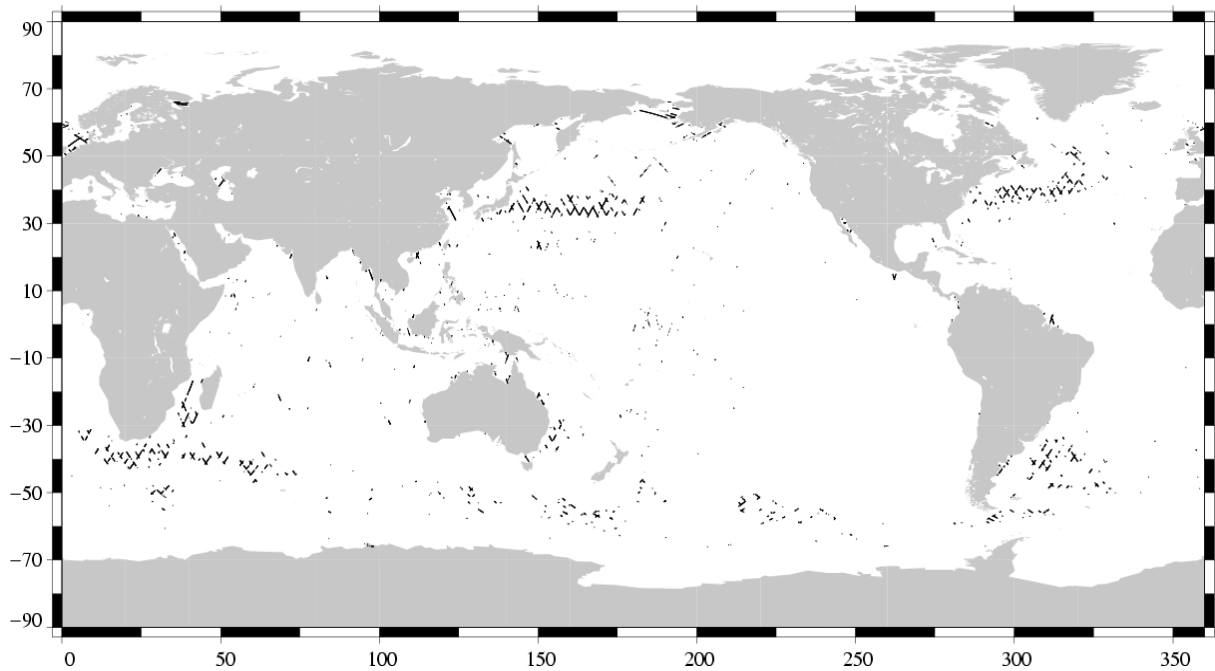
(SSH – MSS) differences greater than 0.3 m TOPEX/Poseidon Cycle 376 (28/11/2002 / 08/12/2002)
