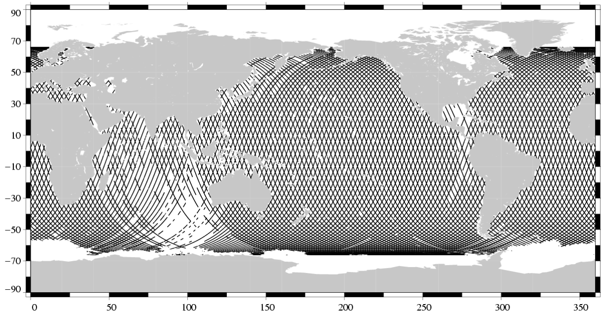
Edited measurements TOPEX Cycle 376 (28/11/2002 / 08/12/2002)
