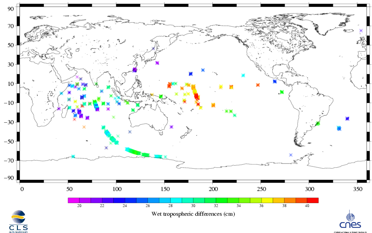
Edited parameter : Radiometer and ECMWF wet tropospheric differences T/P Cycle 376 (28/11/2002 / 08/12/2002)
