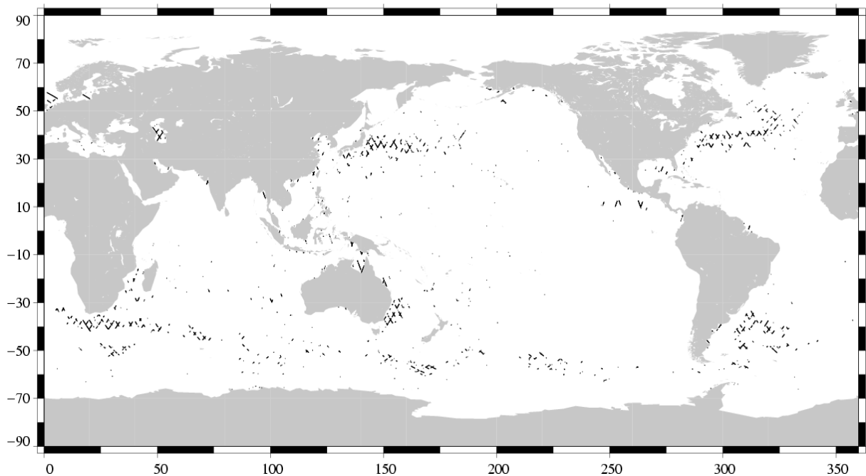
(SSH – MSS) differences greater than 0.3 m TOPEX/Poseidon Cycle 385 (25/02/2003 / 07/03/2003)
