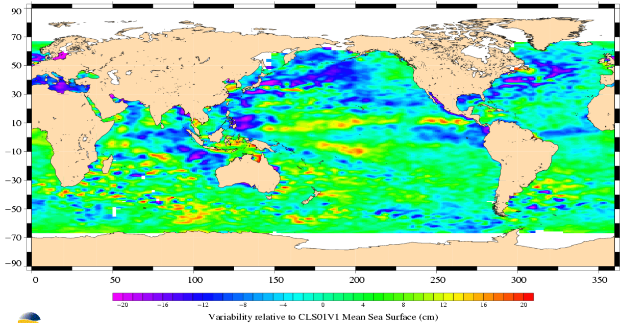
(SSH – MSS) differences greater than 0.3 m TOPEX/Poseidon Cycle 385 (25/02/2003 / 07/03/2003)
