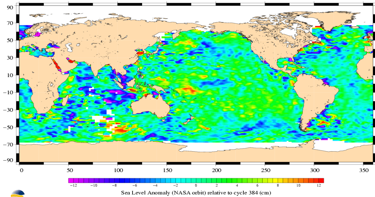
TOPEX/Poseidon, cycle 385 Period : 25/02/2003 – 07/03/2003
