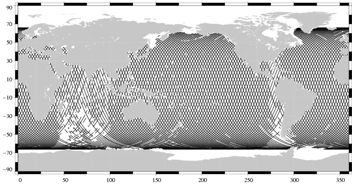
Edited measurements TOPEX Cycle 385 (25/02/2003 / 07/03/2003)
