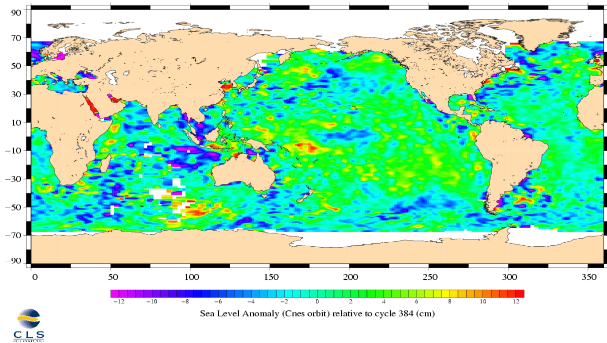
TOPEX/Poseidon, cycle 385 Period : 25/02/2003 – 07/03/2003
