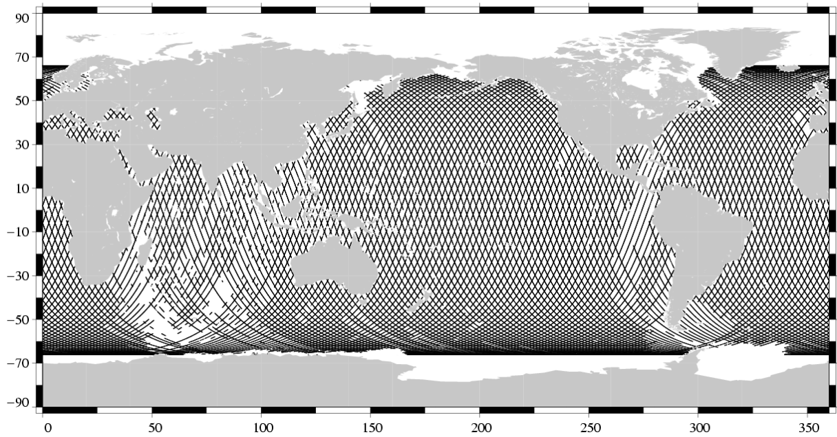
Edited measurements TOPEX Cycle 389 (06/04/2003 / 16/04/2003)
