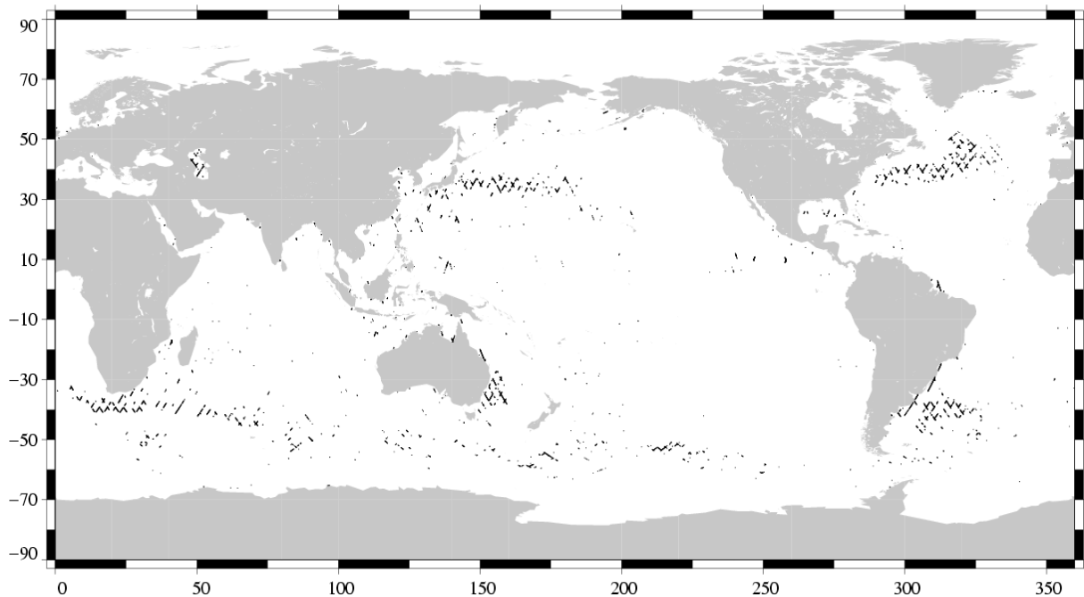
(SSH – MSS) differences greater than 0.3 m TOPEX/Poseidon Cycle 389 (06/04/2003 / 16/04/2003)
