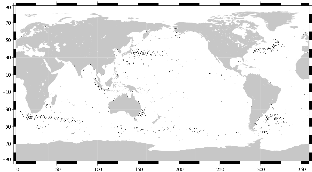
(SSH - MSS) differences greater than 0.3 m TOPEX/Poseidon Cycle 392 (06/05/2003 / 16/05/2003)
