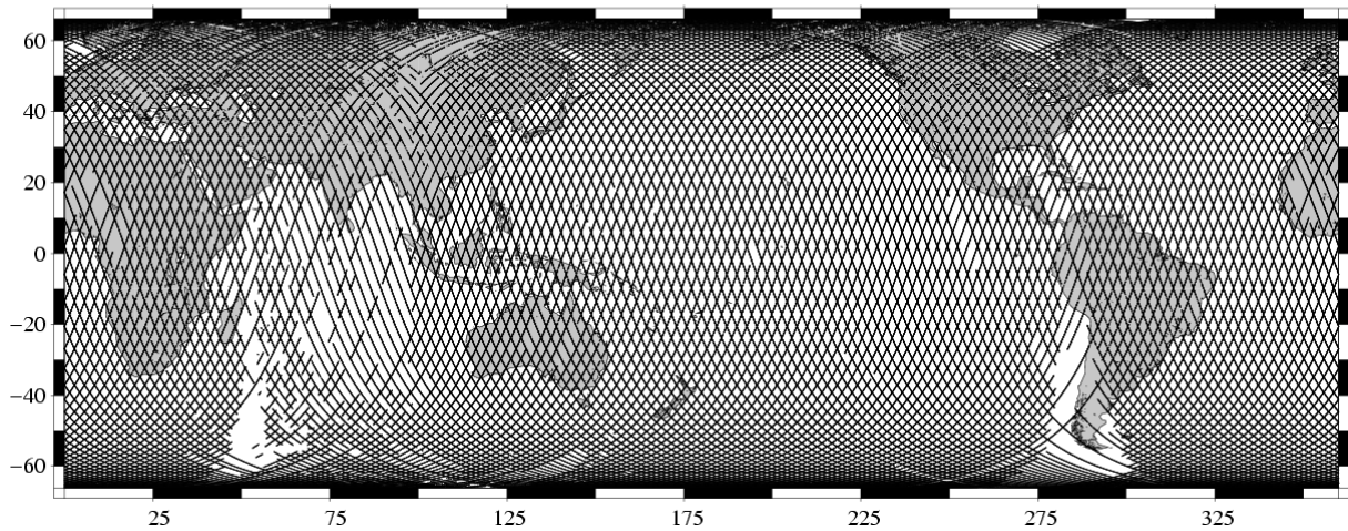
Missing measurements TOPEX/Poseidon Cycle 397 (24/06/2003 / 04/07/2003)
