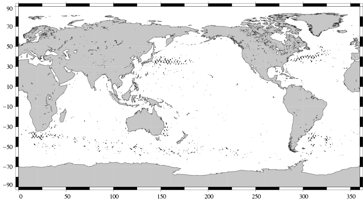
(SSH - MSS) differences greater than 0.3 m TOPEX/Poseidon Cycle 397 (24/06/2003 / 04/07/2003)
