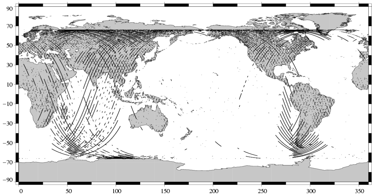
Missing measurements TOPEX/Poseidon Cycle 401 (03/08/2003 / 13/08/2003)
