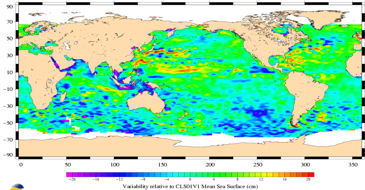
(SSH - MSS) differences greater than 0.3 m TOPEX/Poseidon Cycle 401 (03/08/2003 / 13/08/2003)
