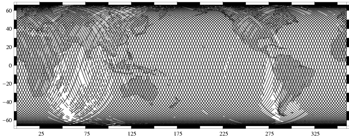
Missing measurements TOPEX/Poseidon Cycle 401 (03/08/2003 / 13/08/2003)
