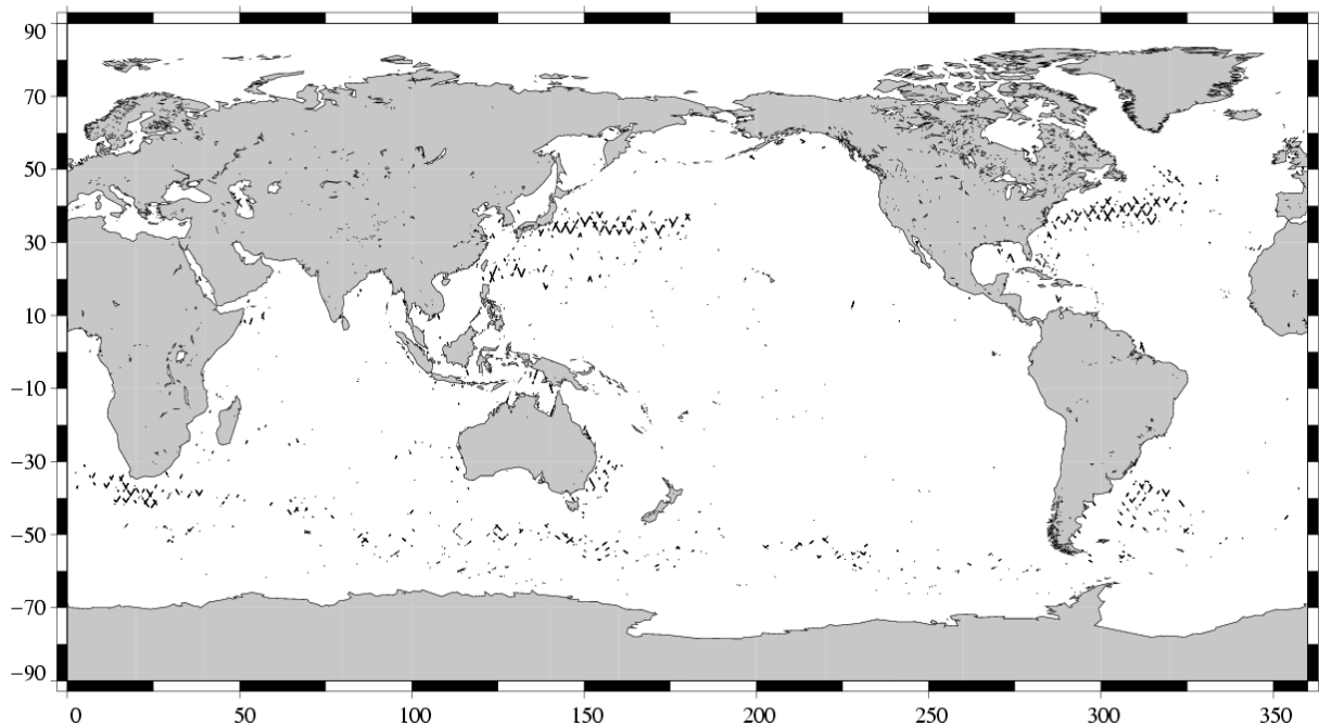
(SSH - MSS) differences greater than 0.3 m TOPEX/Poseidon Cycle 401 (03/08/2003 / 13/08/2003)
