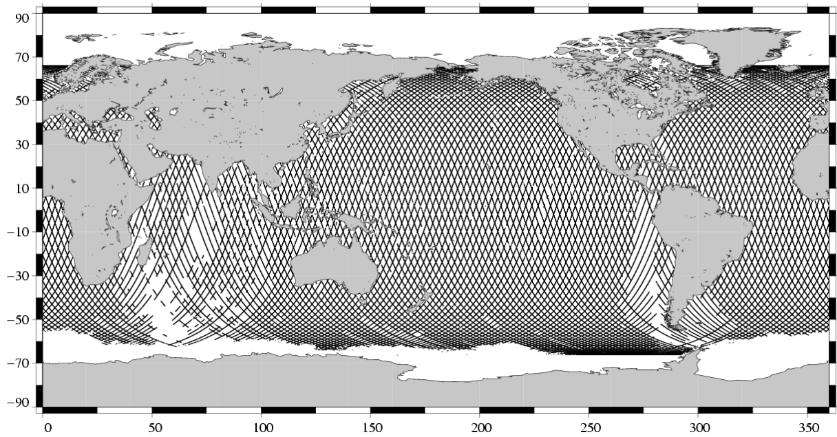
Edited measurements TOPEX Cycle 401 (03/08/2003 / 13/08/2003)
