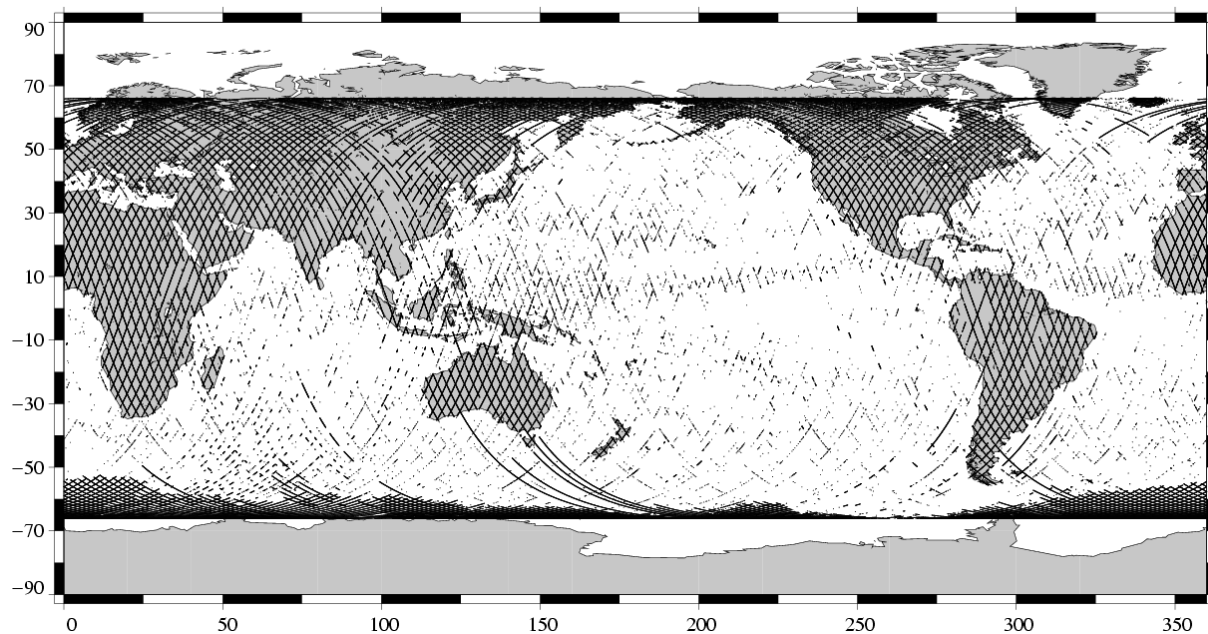
Edited measurements TOPEX Cycle 405 (12/09/2003 / 21/09/2003)
