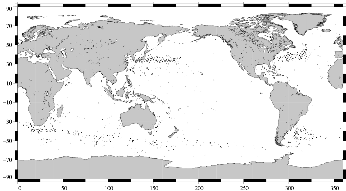
(SSH - MSS) differences greater than 0.3 m TOPEX/Poseidon Cycle 405 (12/09/2003 / 21/09/2003)
