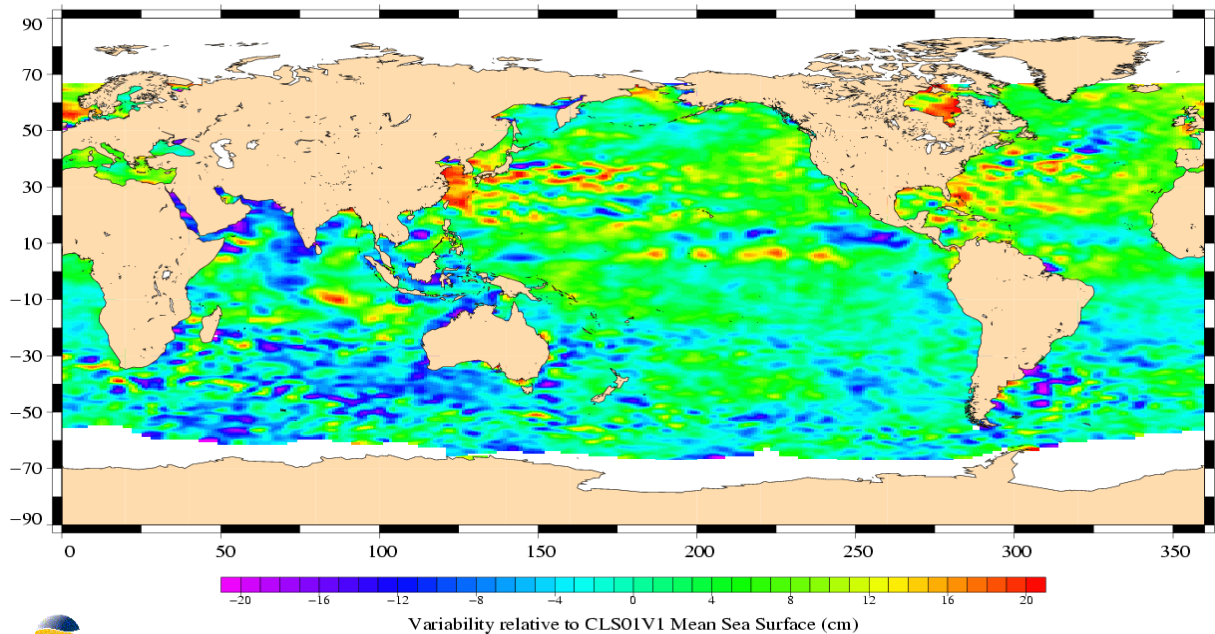
(SSH - MSS) differences greater than 0.3 m TOPEX/Poseidon Cycle 405 (12/09/2003 / 21/09/2003)
