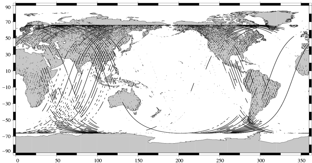
Missing measurements TOPEX/Poseidon Cycle 405 (12/09/2003 / 21/09/2003)
