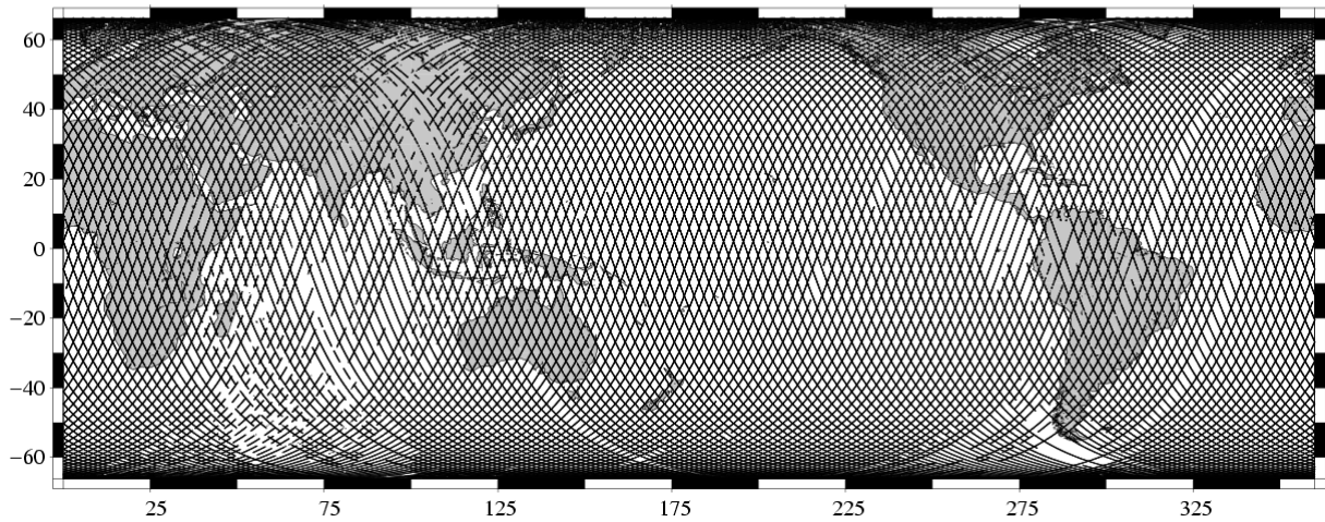
Missing measurements TOPEX/Poseidon Cycle 405 (12/09/2003 / 21/09/2003)
