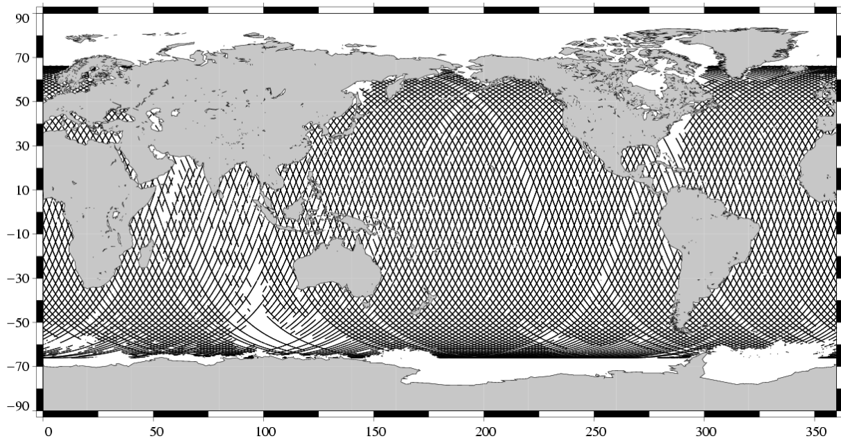
Edited measurements TOPEX Cycle 415 (20/12/2003 / 30/12/2003)
