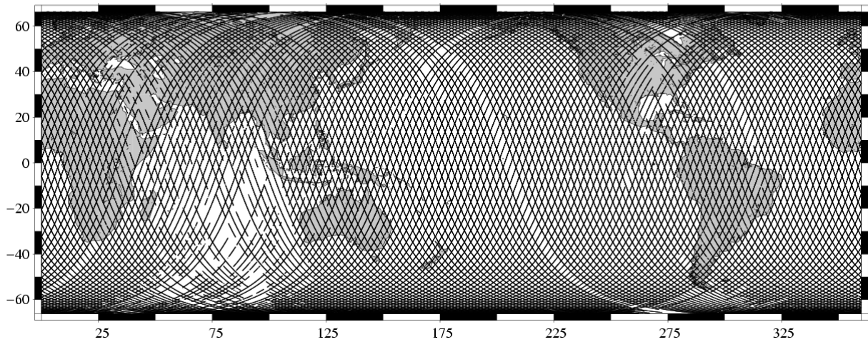
Missing measurements TOPEX/Poseidon Cycle 416 (30/12/2003 / 09/01/2004)
