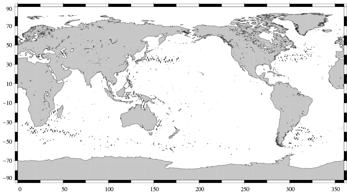
(SSH - MSS) differences greater than 0.3 m TOPEX/Poseidon Cycle 416 (30/12/2003 / 09/01/2004)
