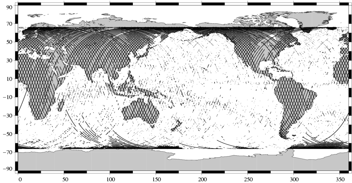
Edited measurements TOPEX Cycle 416 (30/12/2003 / 09/01/2004)
