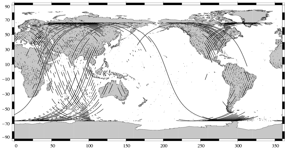
Missing measurements TOPEX/Poseidon Cycle 416 (30/12/2003 / 09/01/2004)
