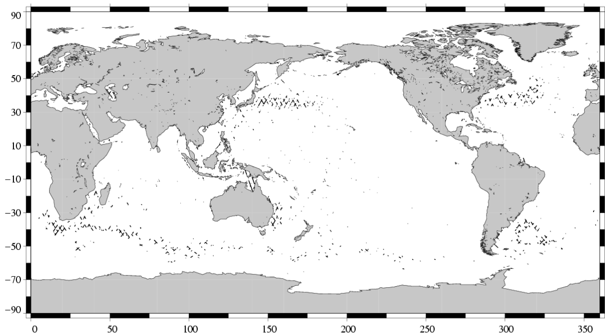
(SSH - MSS) differences greater than 0.3 m TOPEX/Poseidon Cycle 417 (09/01/2004 / 18/01/2004)
