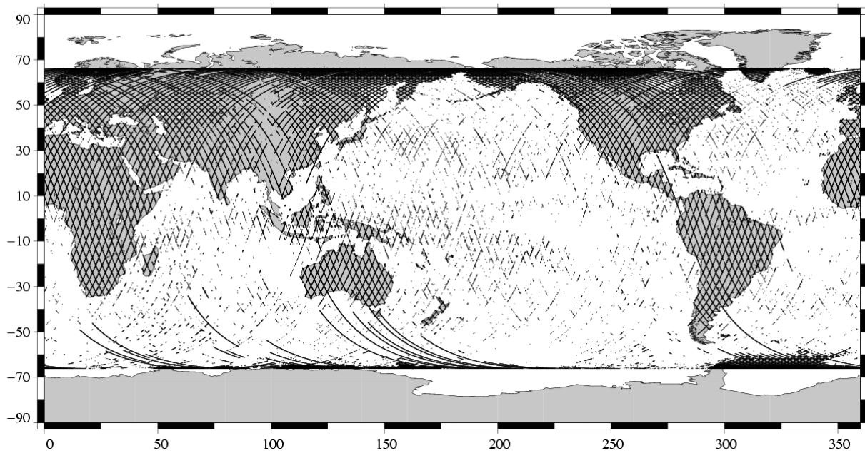
Edited measurements TOPEX Cycle 417 (09/01/2004 / 18/01/2004)
