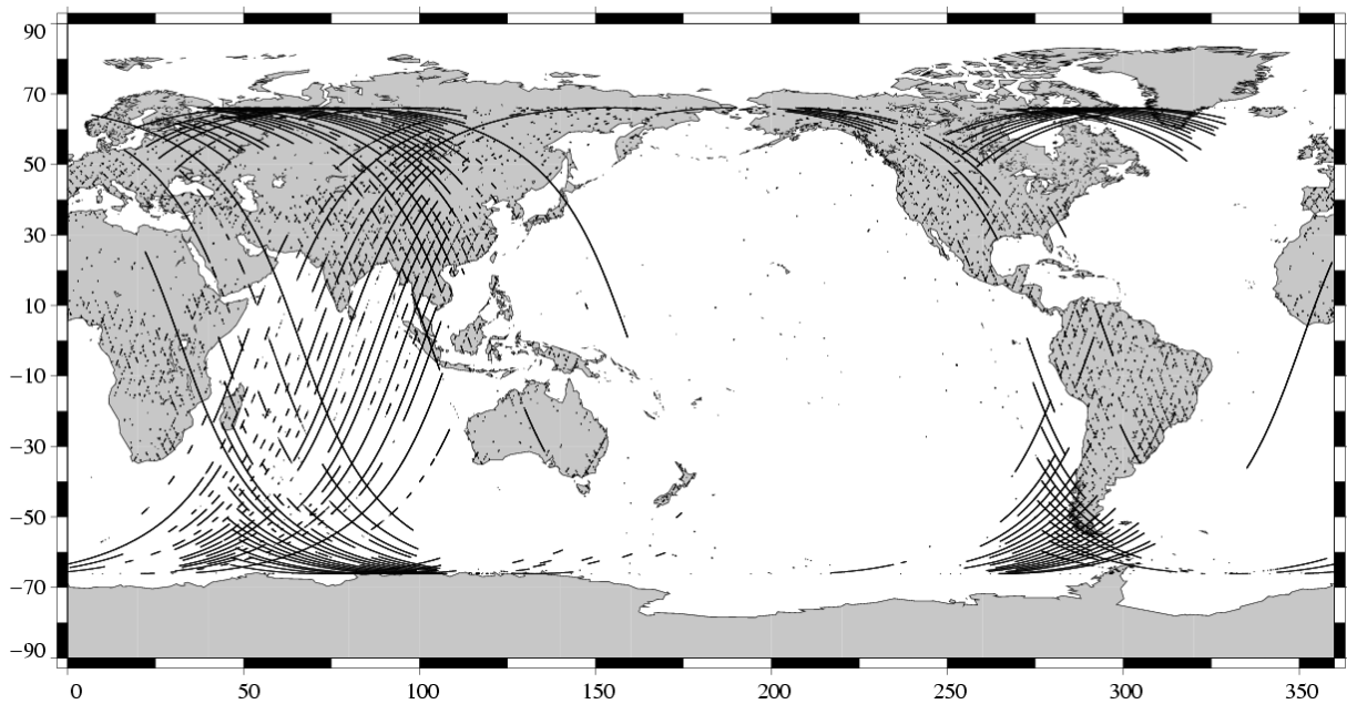
Missing measurements TOPEX/Poseidon Cycle 417 (09/01/2004 / 18/01/2004)
