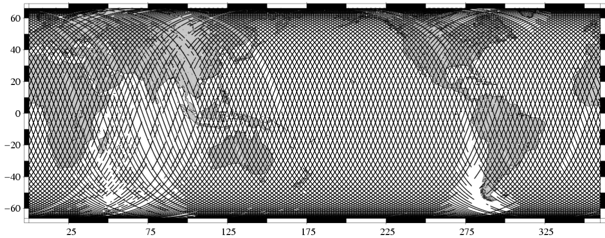
Missing measurements TOPEX/Poseidon Cycle 417 (09/01/2004 / 18/01/2004)
