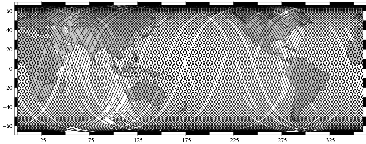
Missing measurements TOPEX/Poseidon Cycle 419 (28/01/2004 / 07/02/2004)
