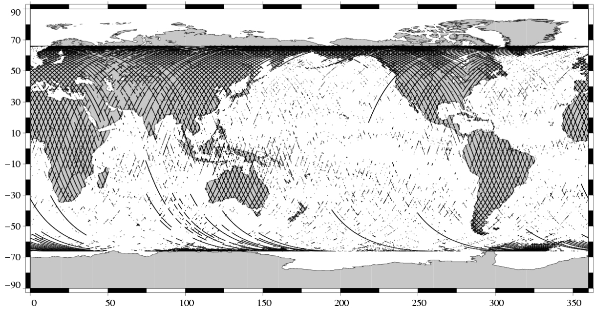
Edited measurements TOPEX Cycle 419 (28/01/2004 / 07/02/2004)
