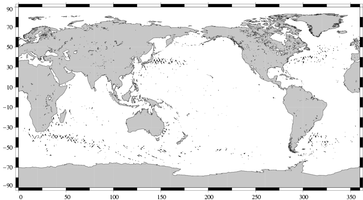
(SSH - MSS) differences greater than 0.3 m TOPEX/Poseidon Cycle 419 (28/01/2004 / 07/02/2004)
