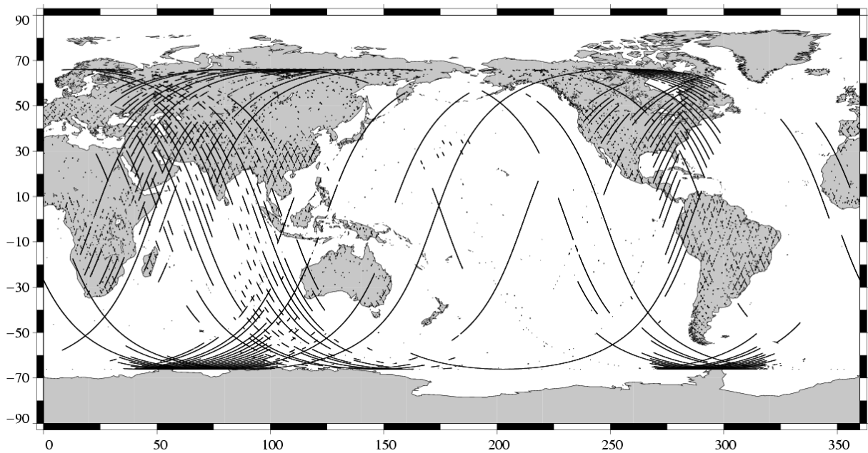
Missing measurements TOPEX/Poseidon Cycle 419 (28/01/2004 / 07/02/2004)
