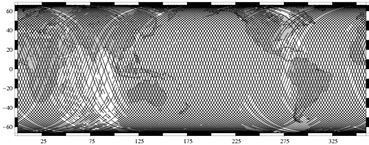
Missing measurements TOPEX/Poseidon Cycle 420 (07/02/2004 / 17/02/2004)
