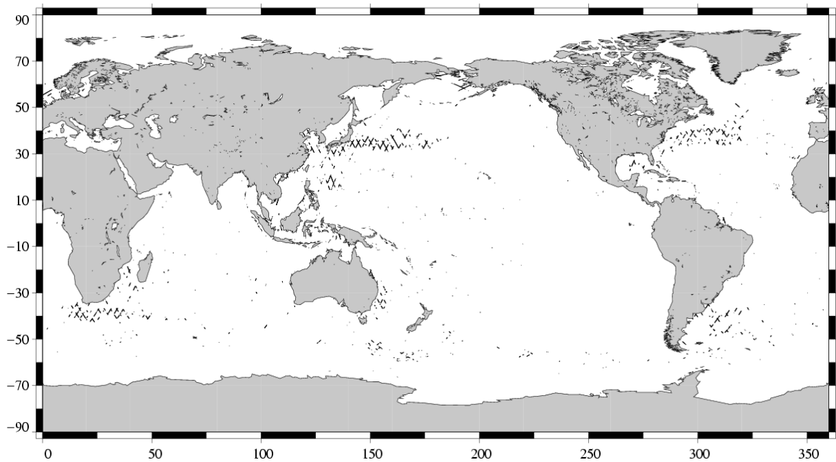
(SSH – MSS) differences greater than 0.3 m TOPEX/Poseidon Cycle 445 (12/10/2004 / 22/10/2004)
