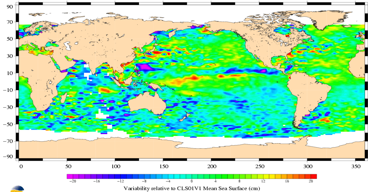
(SSH – MSS) differences greater than 0.3 m TOPEX/Poseidon Cycle 445 (12/10/2004 / 22/10/2004)
