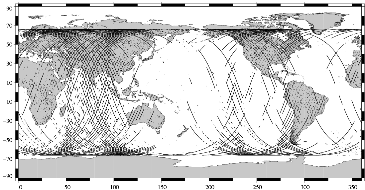
Missing measurements TOPEX/Poseidon Cycle 445 (12/10/2004 / 22/10/2004)
