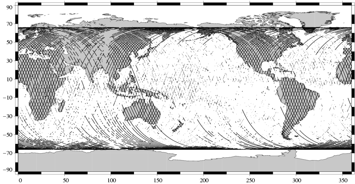
Edited measurements TOPEX Cycle 445 (12/10/2004 / 22/10/2004)
