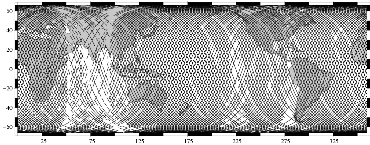
Missing measurements TOPEX/Poseidon Cycle 445 (12/10/2004 / 22/10/2004)
