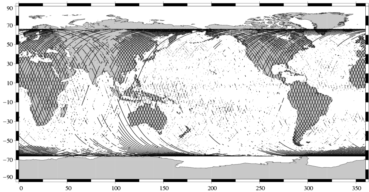
Edited measurements TOPEX Cycle 449 (21/11/2004 / 01/12/2004)
