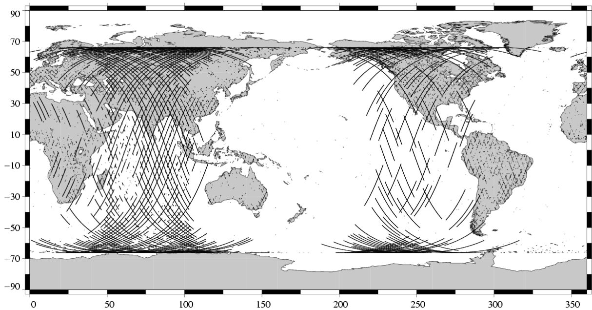
Missing measurements TOPEX/Poseidon Cycle 449 (21/11/2004 / 01/12/2004)
