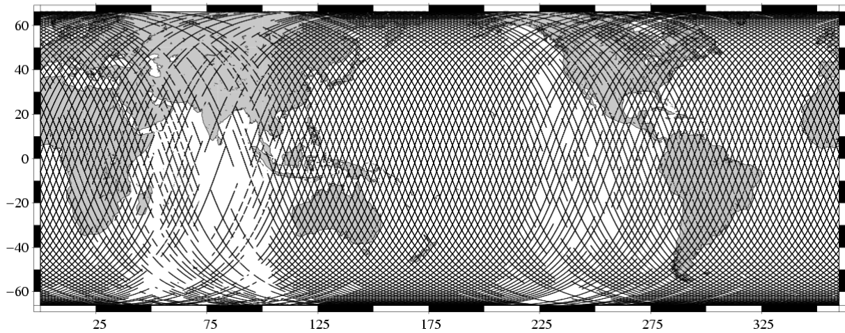
Missing measurements TOPEX/Poseidon Cycle 449 (21/11/2004 / 01/12/2004)
