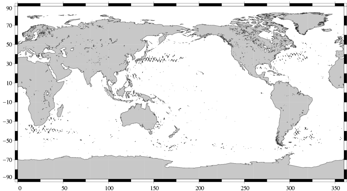
(SSH - MSS) differences greater than 0.3 m TOPEX/Poseidon Cycle 449 (21/11/2004 / 01/12/2004)
