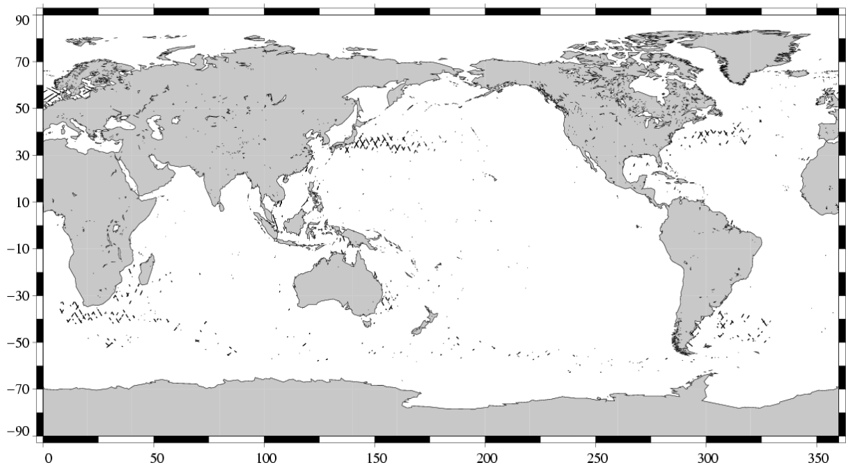
(SSH - MSS) differences greater than 0.3 m TOPEX/Poseidon Cycle 453 (31/12/2004 / 09/01/2005)
