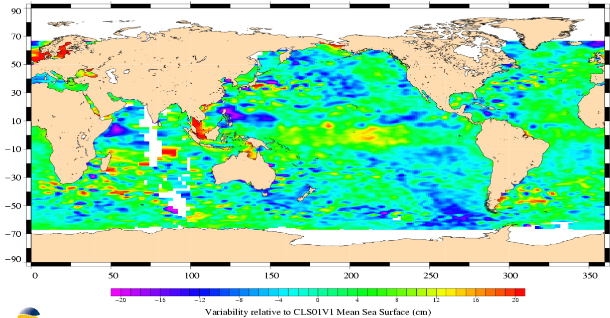
(SSH - MSS) differences greater than 0.3 m TOPEX/Poseidon Cycle 453 (31/12/2004 / 09/01/2005)
