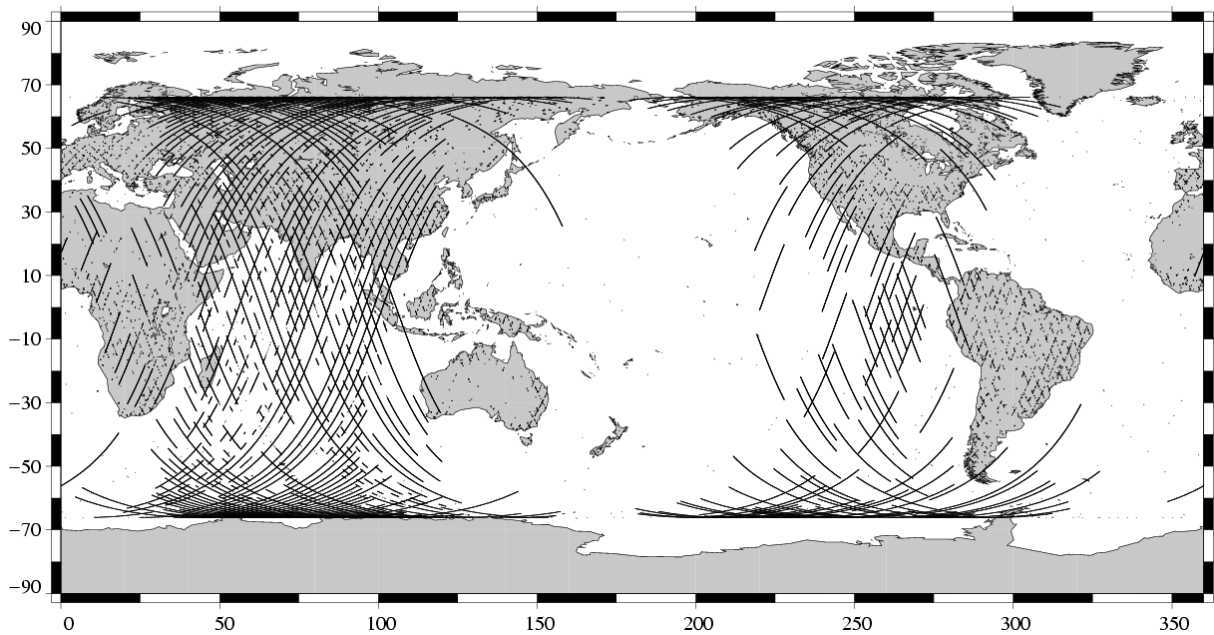
Missing measurements TOPEX/Poseidon Cycle 455 (19/01/2005 / 29/01/2005)
