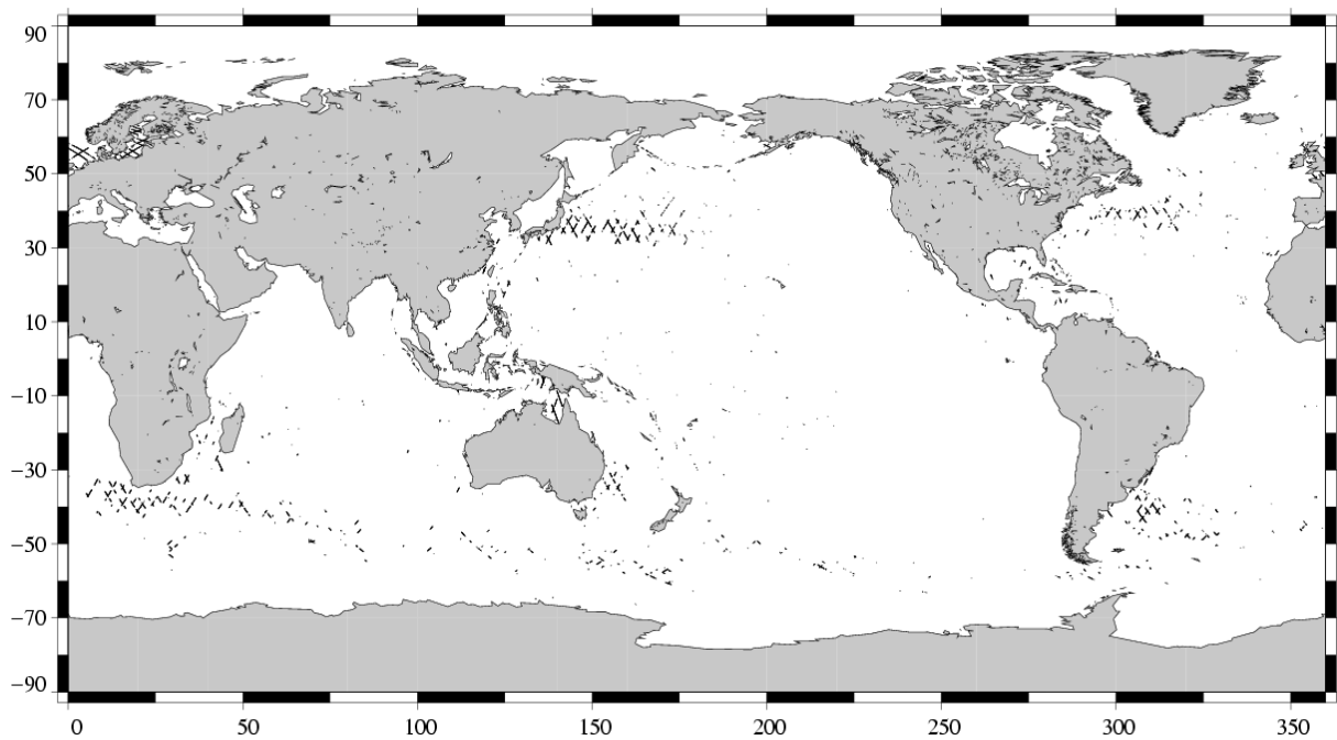
(SSH - MSS) differences greater than 0.3 m TOPEX/Poseidon Cycle 455 (19/01/2005 / 29/01/2005)
