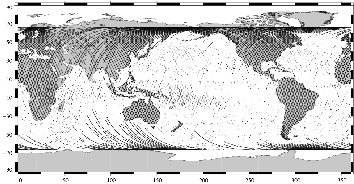
Edited measurements TOPEX Cycle 455 (19/01/2005 / 29/01/2005)
