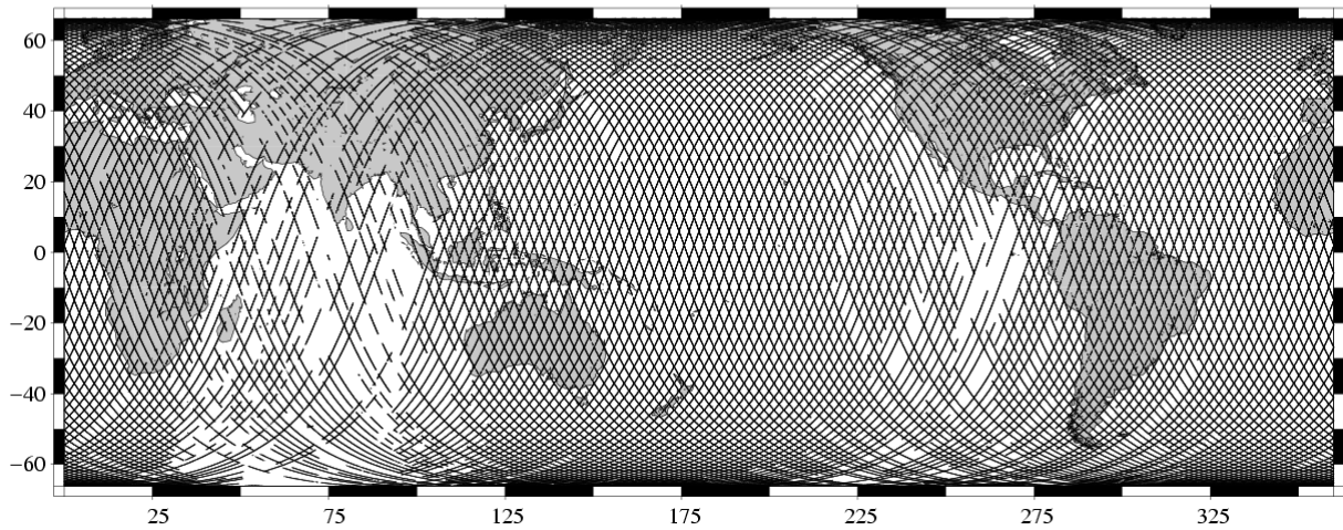
Missing measurements TOPEX/Poseidon Cycle 455 (19/01/2005 / 29/01/2005)
