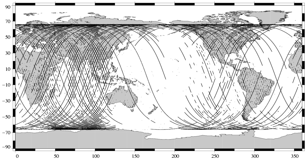
Missing measurements TOPEX/Poseidon Cycle 459 (28/02/2005 / 10/03/2005)
