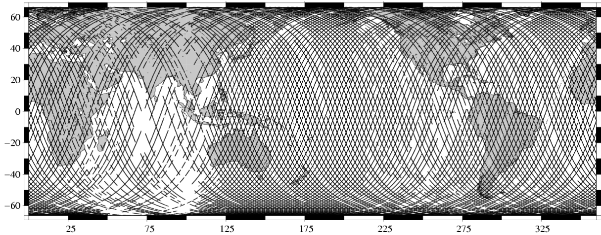
Missing measurements TOPEX/Poseidon Cycle 459 (28/02/2005 / 10/03/2005)
