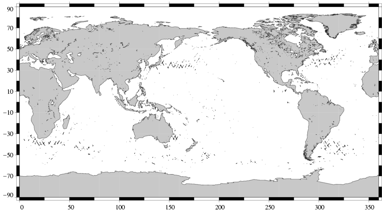
(SSH - MSS) differences greater than 0.3 m TOPEX/Poseidon Cycle 459 (28/02/2005 / 10/03/2005)
