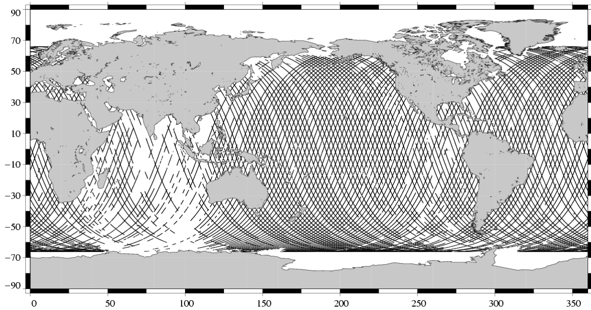
Edited measurements TOPEX Cycle 459 (28/02/2005 / 10/03/2005)
