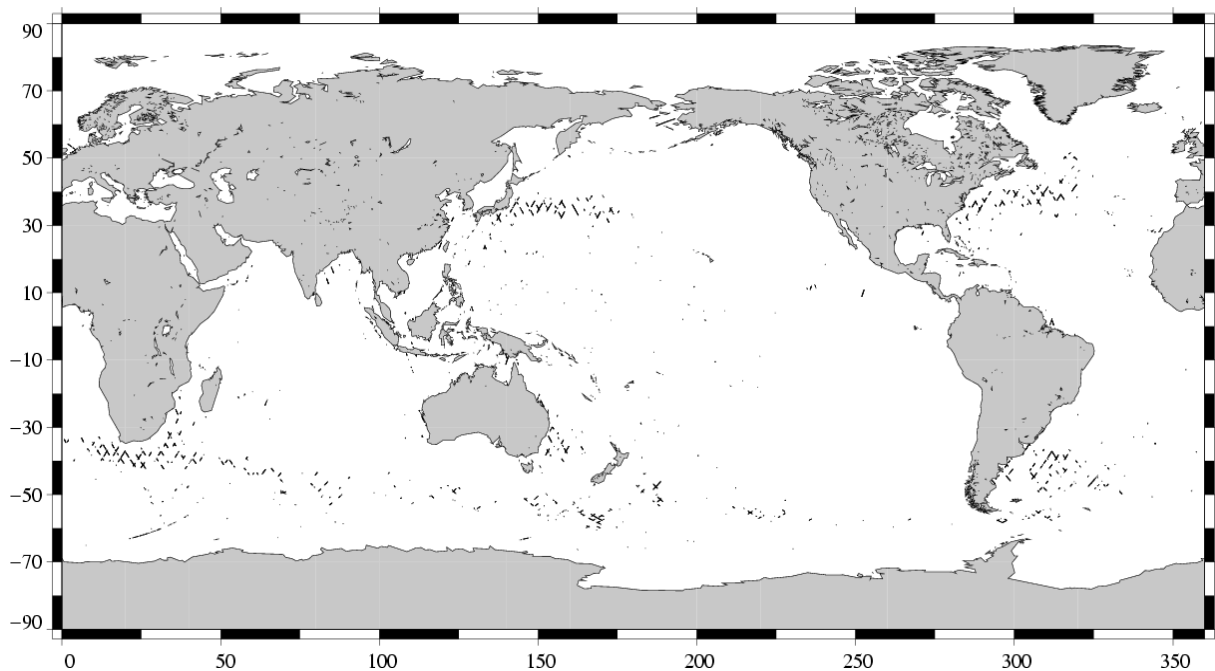
(SSH - MSS) differences greater than 0.3 m TOPEX/Poseidon Cycle 467 (18/05/2005 / 28/05/2005)
