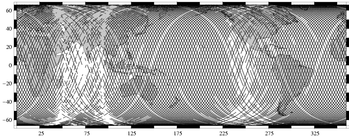
Missing measurements TOPEX/Poseidon Cycle 467 (18/05/2005 / 28/05/2005)
