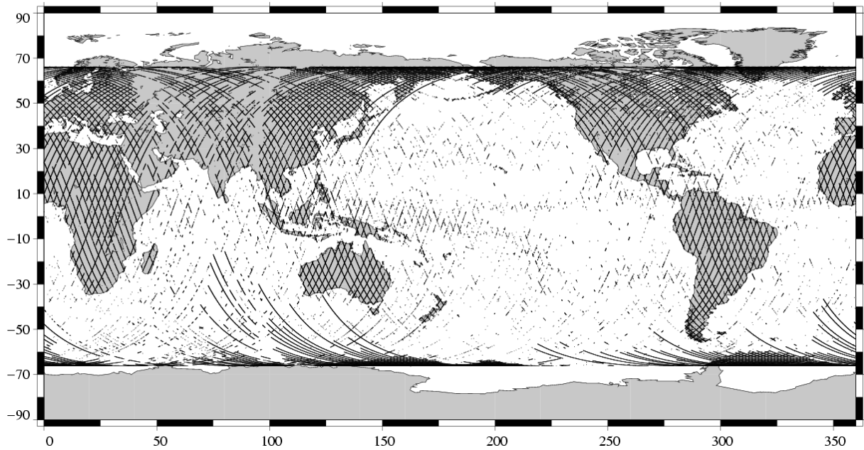
Edited measurements TOPEX Cycle 467 (18/05/2005 / 28/05/2005)
