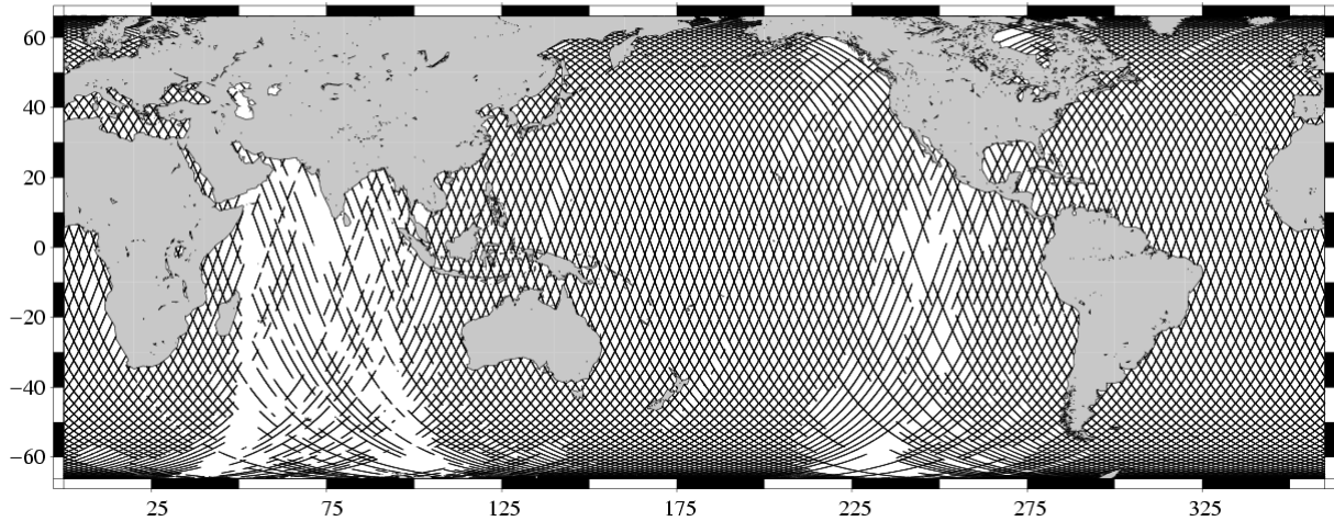
Missing measurements TOPEX/Poseidon Cycle 474 (27/07/2005 / 06/08/2005)
