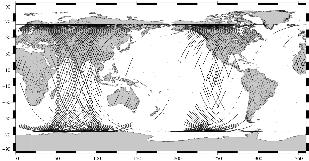
Missing measurements TOPEX/Poseidon Cycle 474 (27/07/2005 / 06/08/2005)
