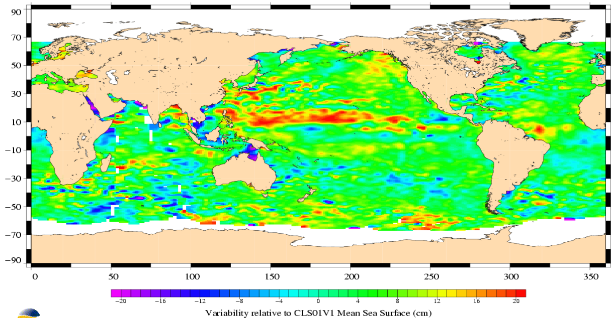
(SSH - MSS) differences greater than 0.3 m TOPEX/Poseidon Cycle 474 (27/07/2005 / 06/08/2005)
