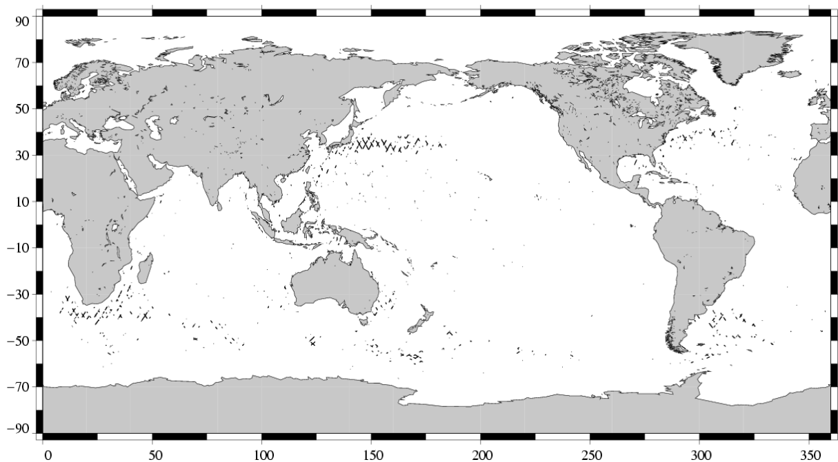
(SSH - MSS) differences greater than 0.3 m TOPEX/Poseidon Cycle 474 (27/07/2005 / 06/08/2005)
