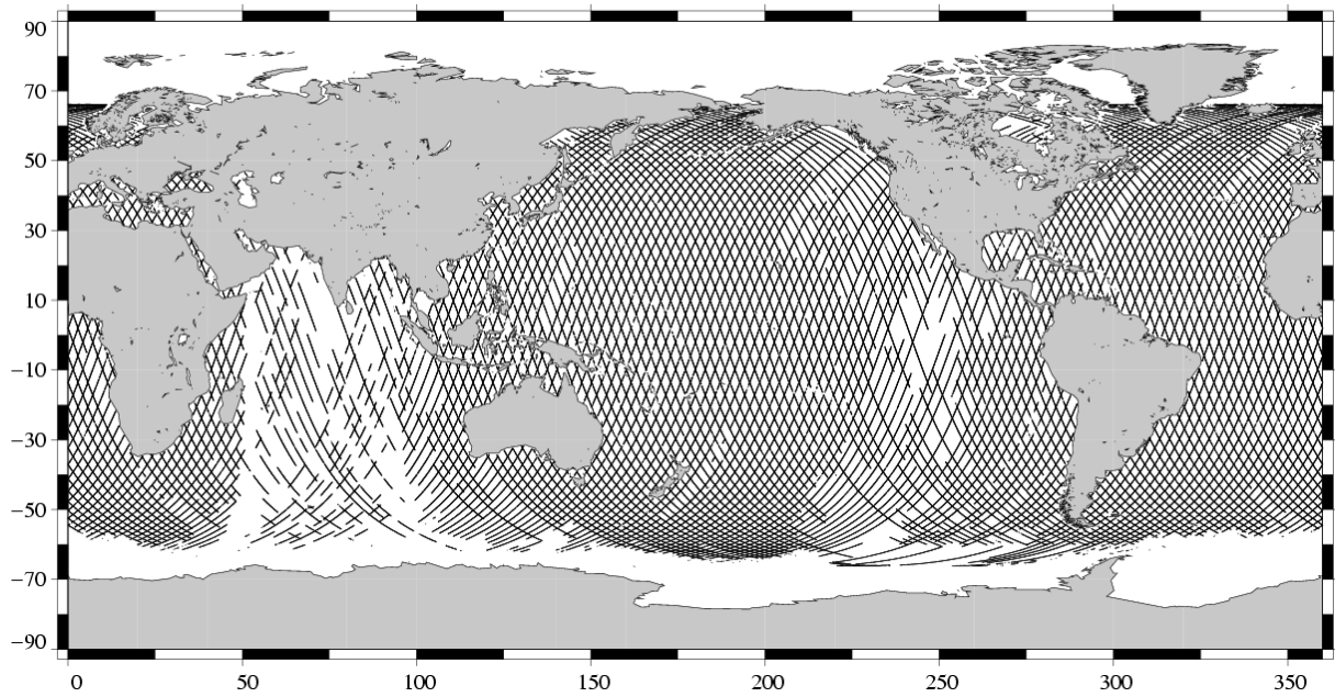
Edited measurements TOPEX Cycle 474 (27/07/2005 / 06/08/2005)
