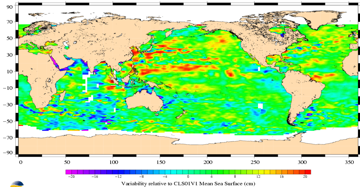
(SSH - MSS) differences greater than 0.3 m TOPEX/Poseidon Cycle 478 (04/09/2005 / 14/09/2005)
