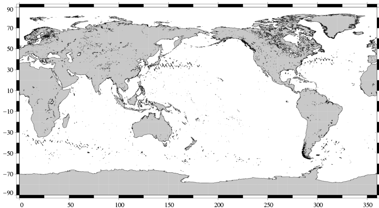
(SSH - MSS) differences greater than 0.3 m TOPEX/Poseidon Cycle 478 (04/09/2005 / 14/09/2005)
