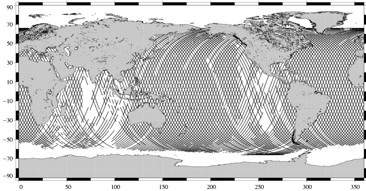
Edited measurements TOPEX Cycle 478 (04/09/2005 / 14/09/2005)
