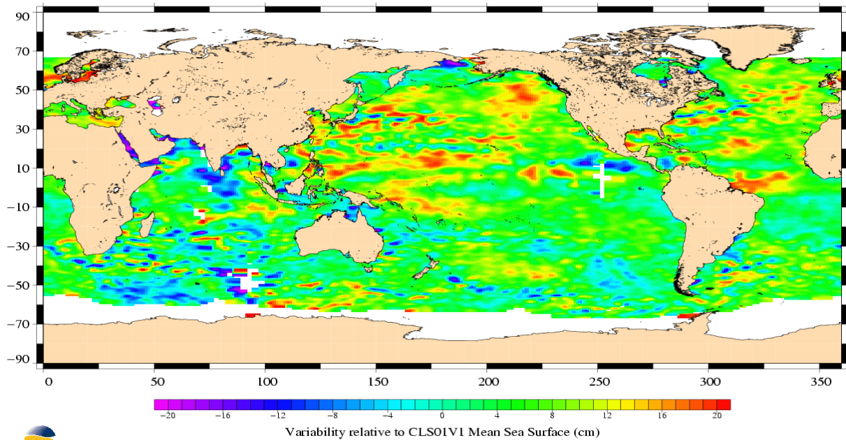
(SSH - MSS) differences greater than 0.3 m TOPEX/Poseidon Cycle 479 (14/09/2005 / 24/09/2005)
