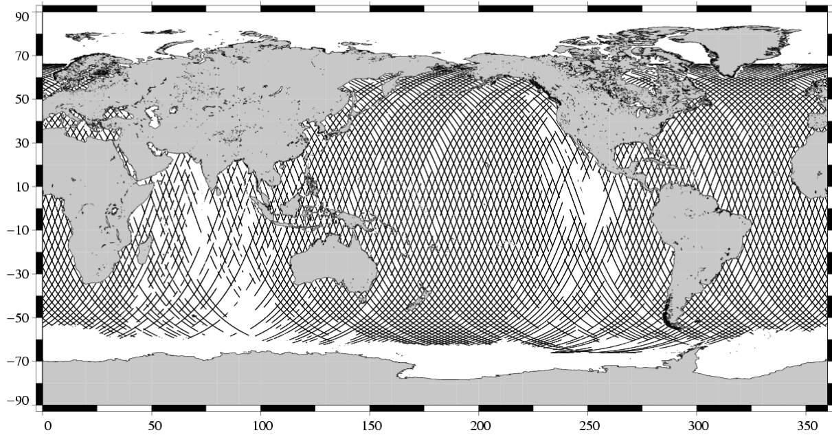
Edited measurements TOPEX Cycle 479 (14/09/2005 / 24/09/2005)
