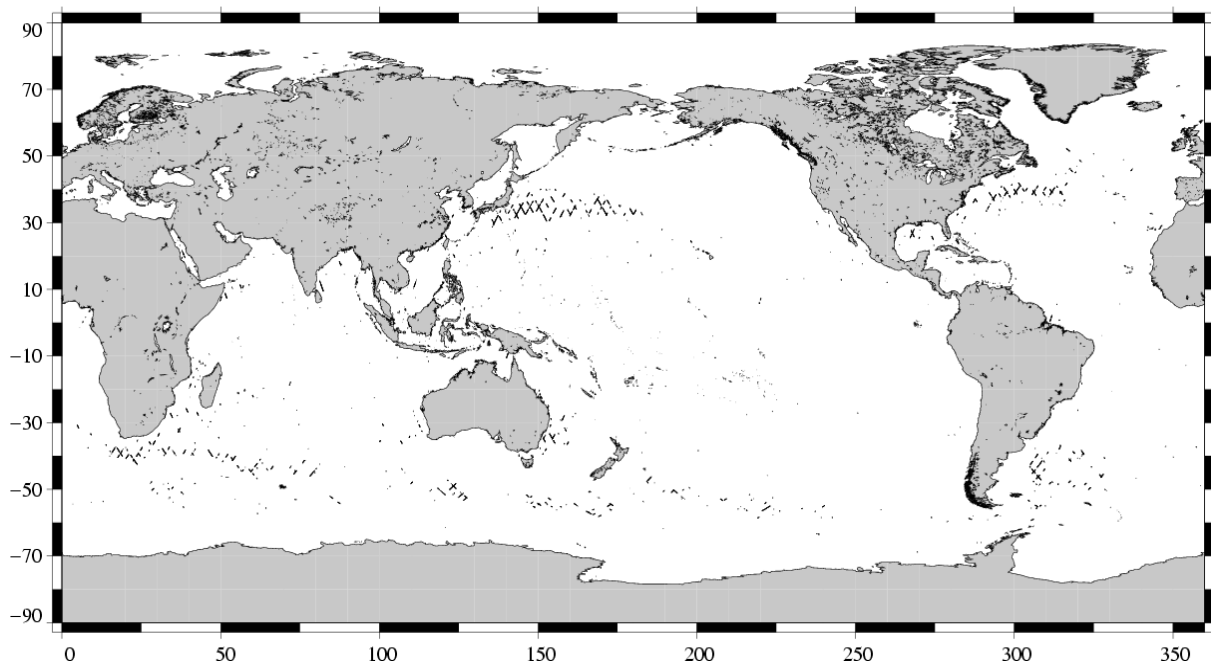
(SSH - MSS) differences greater than 0.3 m TOPEX/Poseidon Cycle 479 (14/09/2005 / 24/09/2005)
