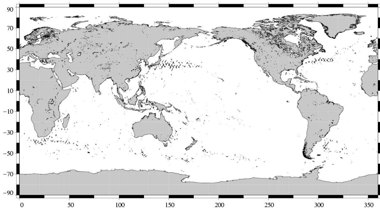
(SSH - MSS) differences greater than 0.3 m TOPEX/Poseidon Cycle 480 (24/09/2005 / 04/10/2005)
